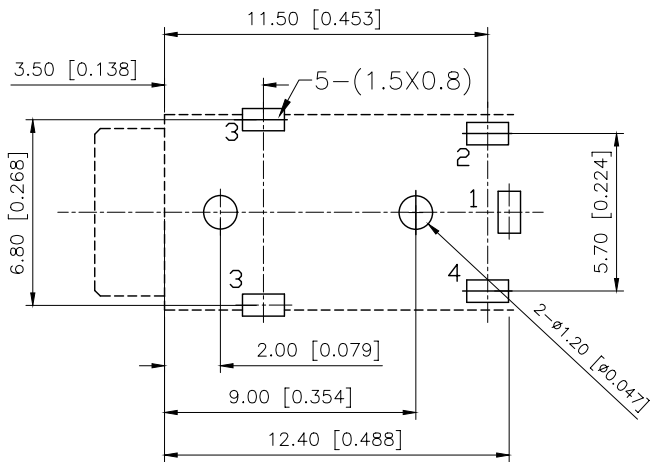
PCB Layout
