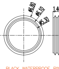
BLACK WATERPROOF RING
