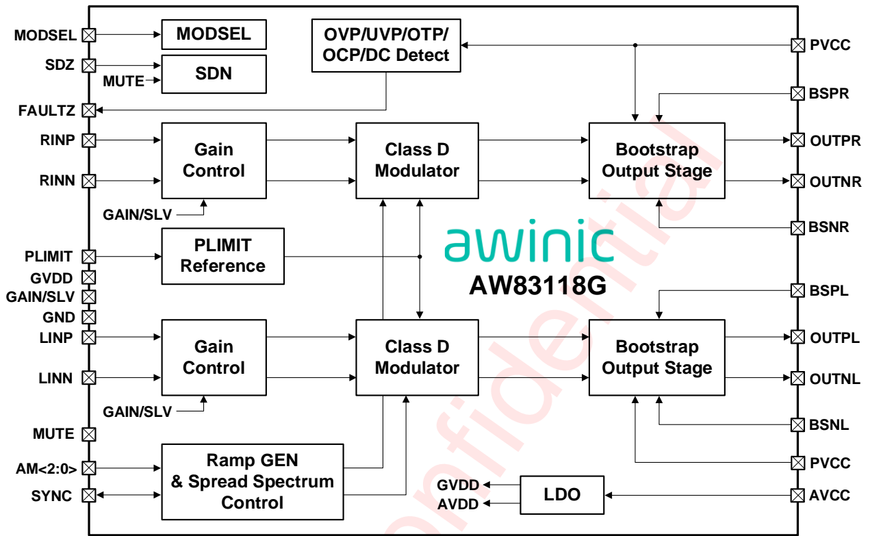
Figure 3 AW83118G Functional Diagram
