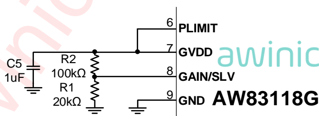
Figure 6 Gain, Master/Slave
