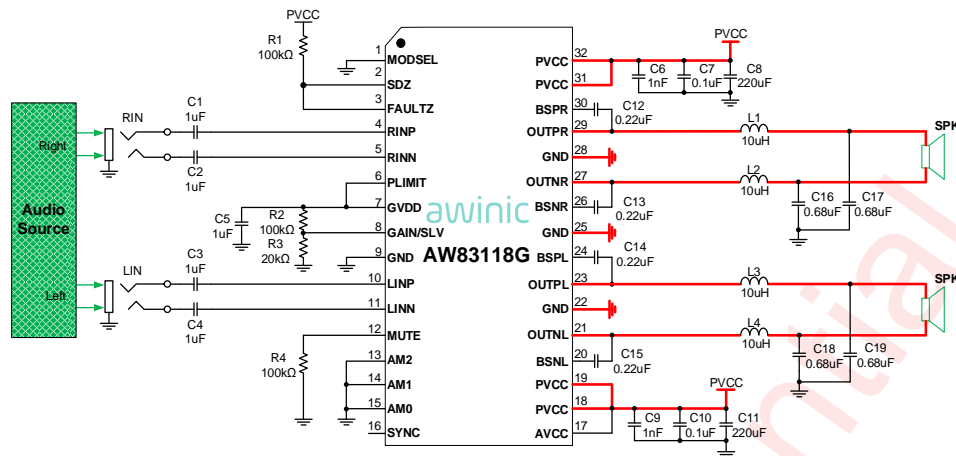
Figure 4 AW83118G Typical Application Diagram
