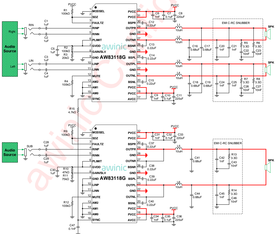
Figure 5 AW83118G 2.1 Master and Slave Application Diagram
