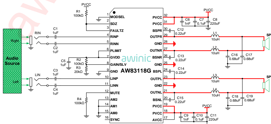
Figure 1 Typical Application Circuit of AW83118G
