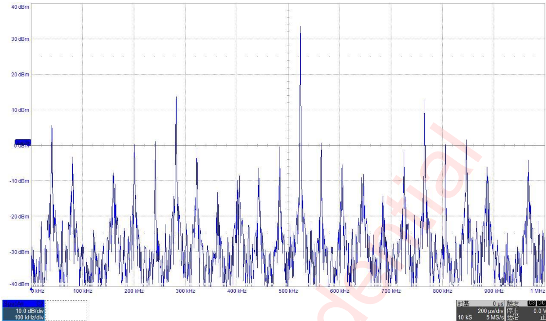
Figure 12 AM<2:0>=001, fsw=500kHz, Output spectrum of the AW83118G
