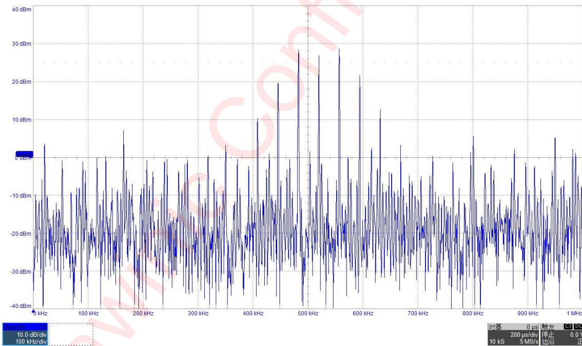
Figure 13 AM<2:0>=110, fsw=500kHz±12%, Output spectrum of the AW83118G
