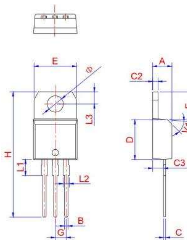
TO-220B Non-Ins
