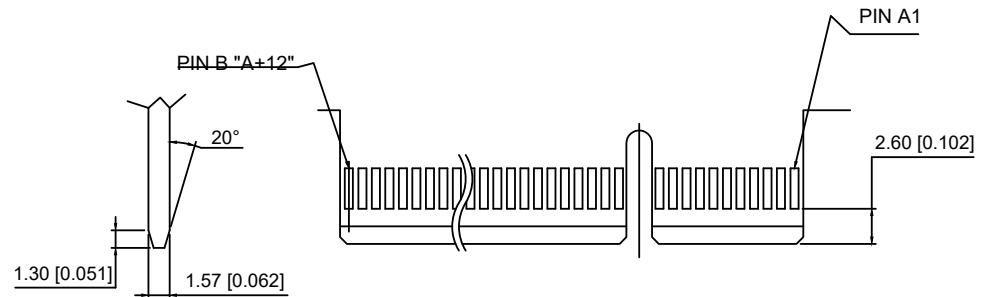
SECONDARY (SOLDER) SIDE
