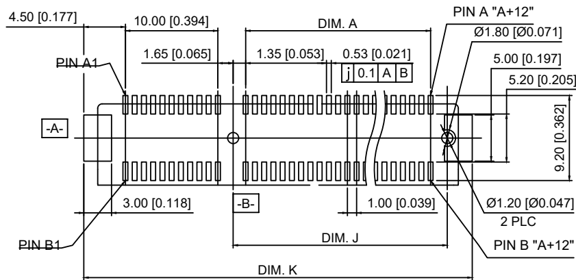
RECOMMENDED PCB LAYOUT (COMPONENT SIDE) TOLERANCE: ±0.05
