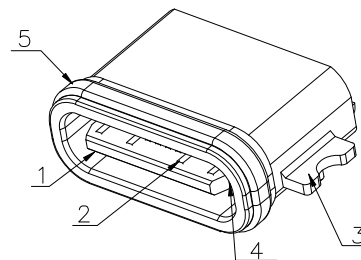
3D VIEW
