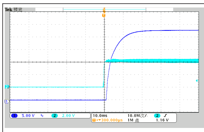
图 6: ON/OFF 启机延时, Vin=24V, Io=2.7A, TC=25°C CH1: 输出电压, CH2: ON/OFF 电压
