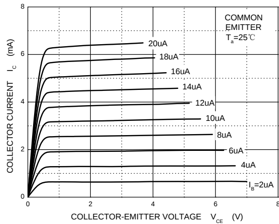
Static Characteristic
