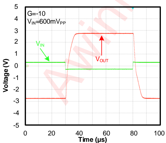
Figure 33 Overload Recovery
