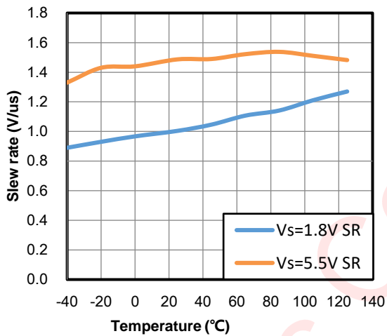
Figure 31 SR vs. Temperature
