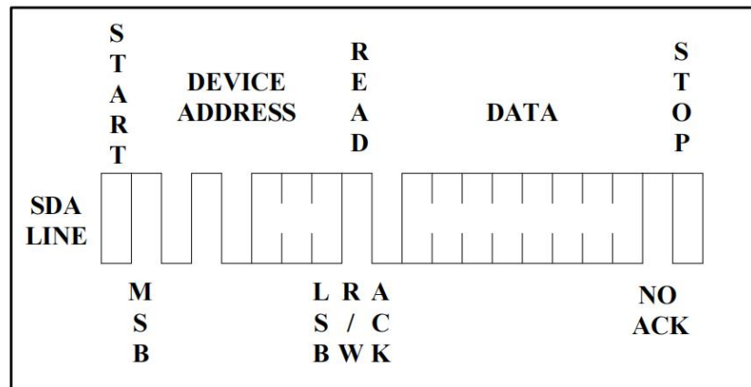
Figure 9. Random Read
