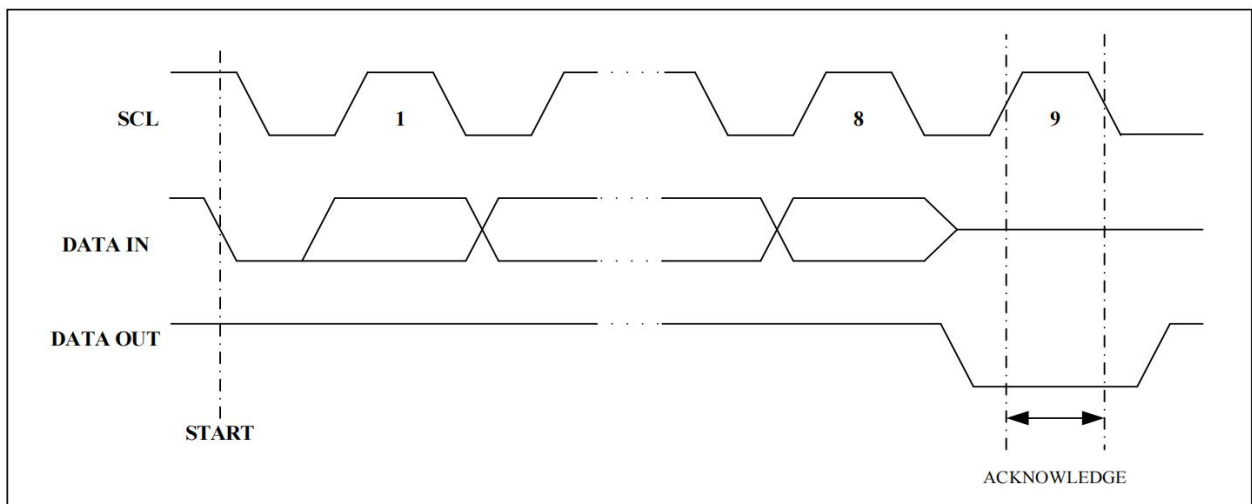
Figure 4. Output Acknowledge
