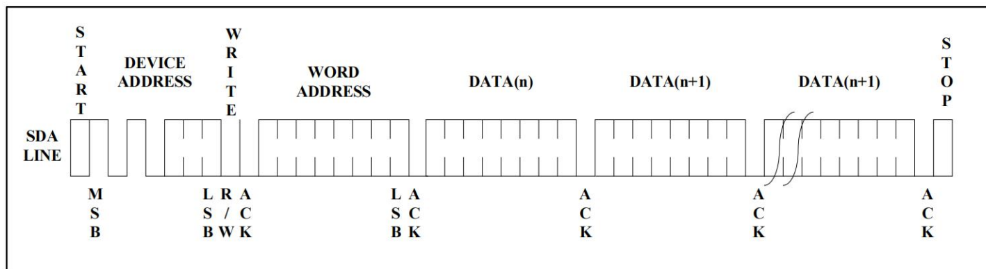
Figure 7. Page Write
