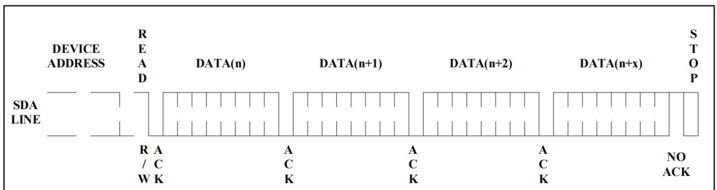
Figure 10. Sequential Read
