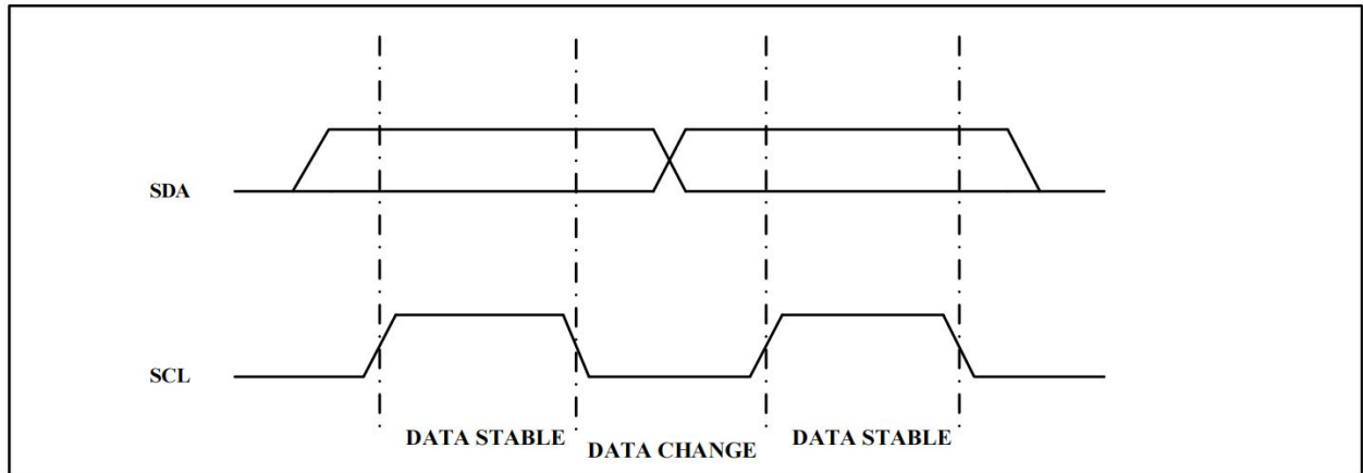
Figure 2. Data Validity
