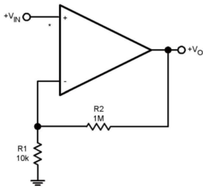
Non Inverting DC Gain (0V Input =0V Output)
