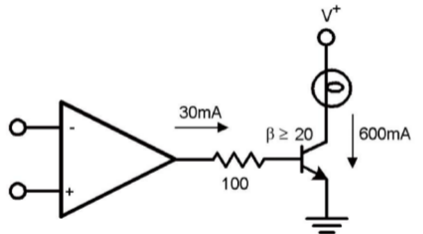
Lamp Driver
