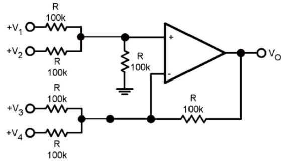
Dc Summing Amplifier(V)
