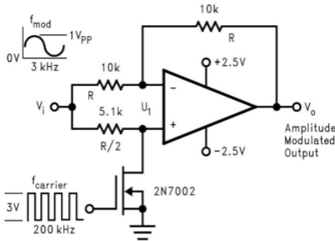
Amplitude Modulator Circuit
