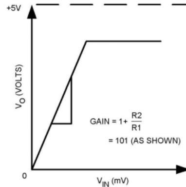
Non Inverting DC Gain (0V Input =0V Output)
