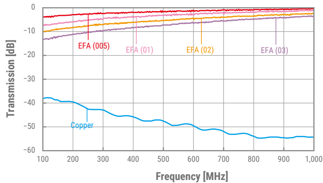
FF1 – Attenuation of Transmission Noise
