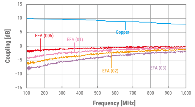
FF1 – Attenuation of Coupling Noise
