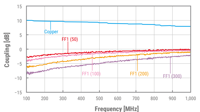
EFF4 – Attenuation of Coupling Noise
