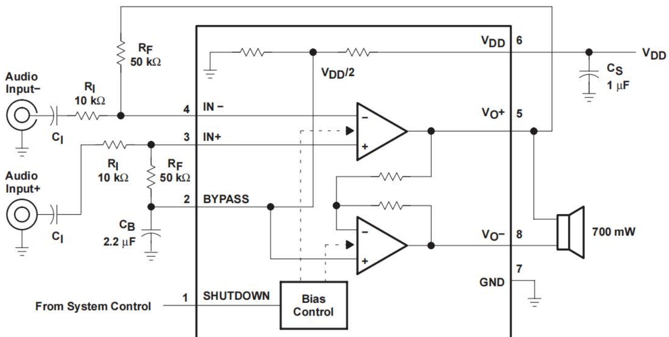
Figure 27. TPA731 Application Circuit With Differential Input
