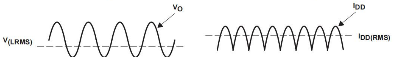
Figure 25. Voltage and Current Waveforms for BTL Amplifiers
