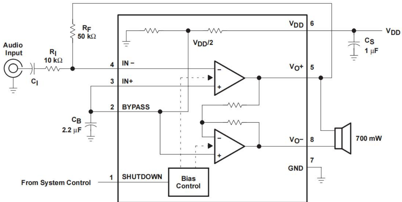
Figure 26. TPA731 Application Circuit
