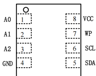
8-pad DFN
