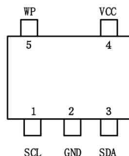
5-lead SOT23-5
