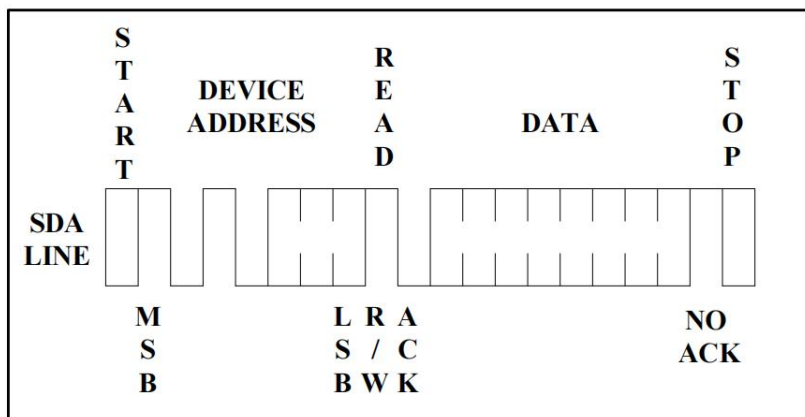
Figure 9. Random Read
