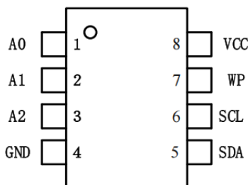
8-lead SOP
