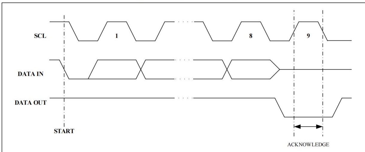
Figure 4. Output Acknowledge
