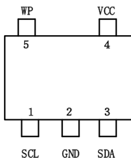
5-lead TSOT23-5
