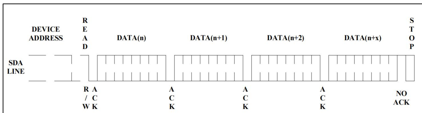
Figure 10. Sequential Read
