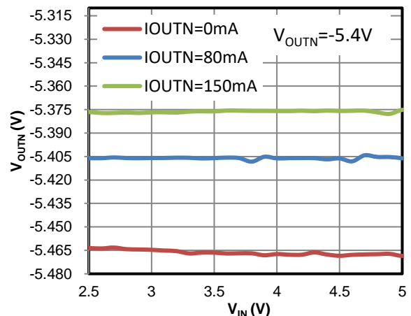
Figure 28 Line Regulation (150mA Mode)
