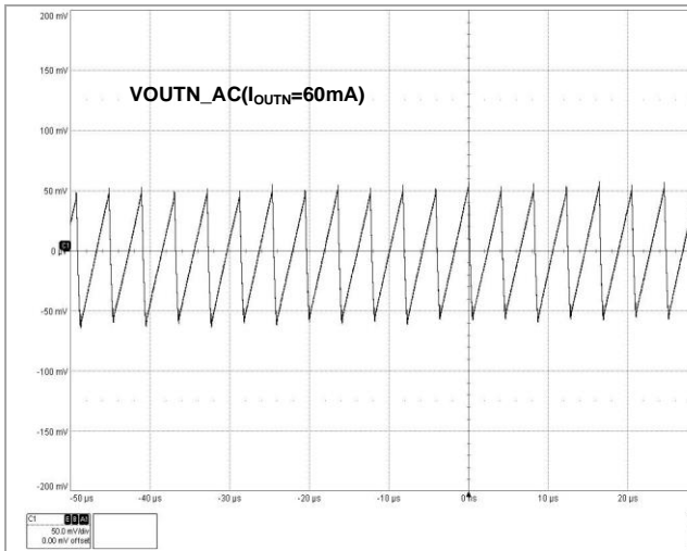
Figure 59 V OUTN Output Voltage Ripple(150mA Mode)
