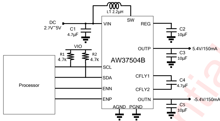
Figure 4 AW37504B Application circuit
