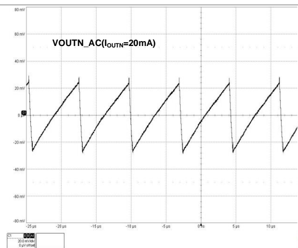
Figure 52 V OUTN Output Voltage Ripple (80mA Mode)
