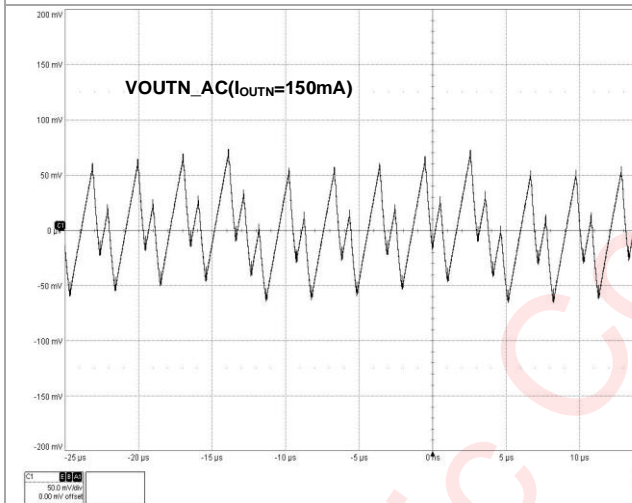
Figure 61 V OUTN Output Voltage Ripple(150mA Mode)
