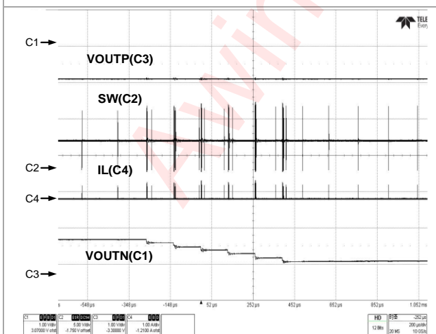
Figure 99 Ramp Up (V OUTN )
