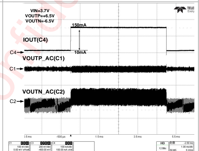
Figure 74 Load Transient(150mA Mode)
