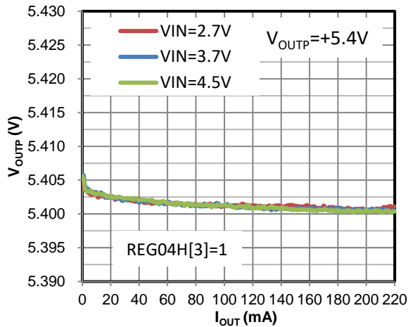
Figure 47 Load Regulation (150mA Mode)
