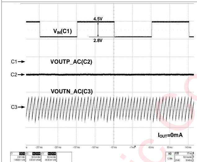
Figure 79 Line Transient (80mA Mode)
