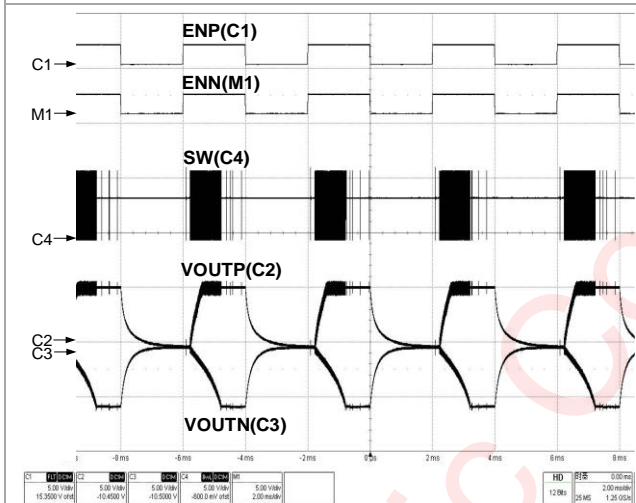
Figure 97 Power Up/Down With Active Discharge
