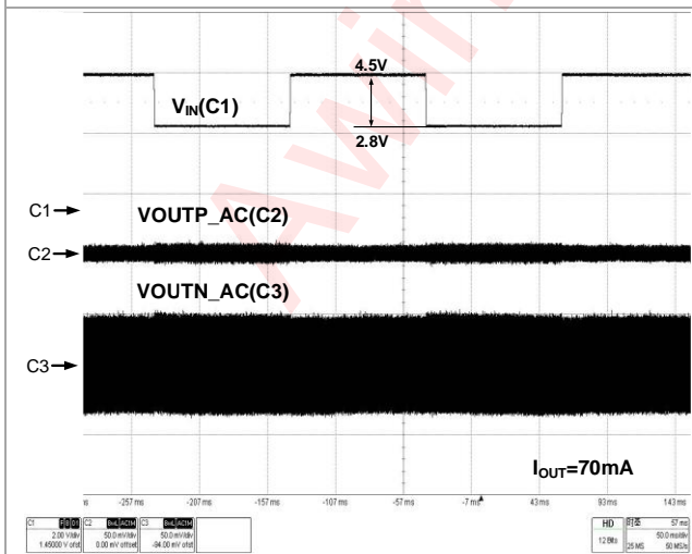
Figure 81 Line Transient (80mA Mode)
