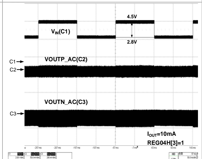
Figure 86 Line Transient (150mA Mode)
