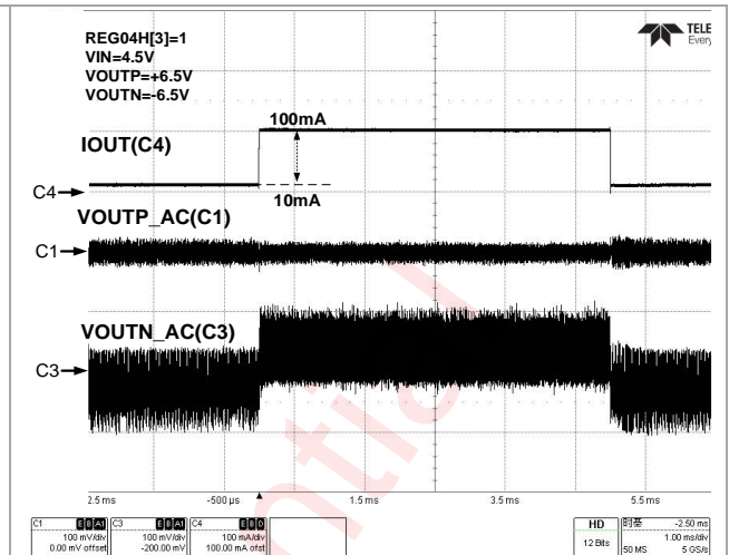
Figure 72 Load Transient(80mA Mode)
