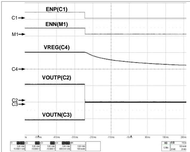
Figure 95 Power Down Sequencing (Simultaneous)
