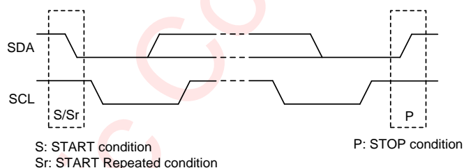
Figure 104 I 2 C Start/Stop Condition Timing
