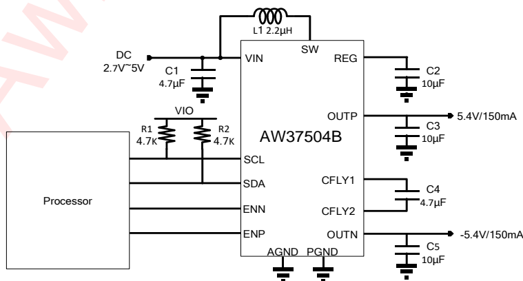
Figure 1 Typical Application Circuit of AW37504B
