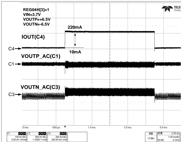
Figure 77 Load Transient(150mA Mode)
