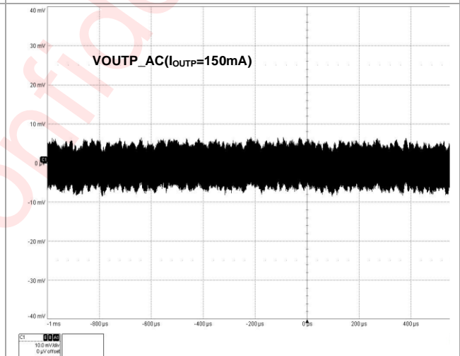
Figure 62 V OUTP Output Voltage Ripple(150mA Mode)
