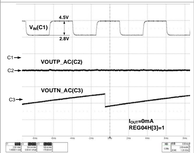
Figure 82 Line Transient (80mA Mode)
