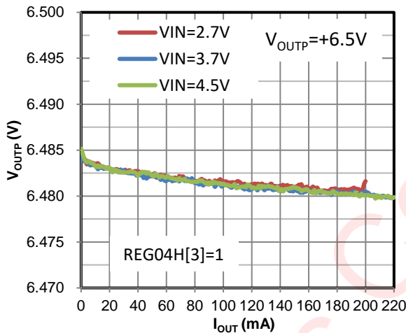
Figure 49 Load Regulation (150mA Mode)
