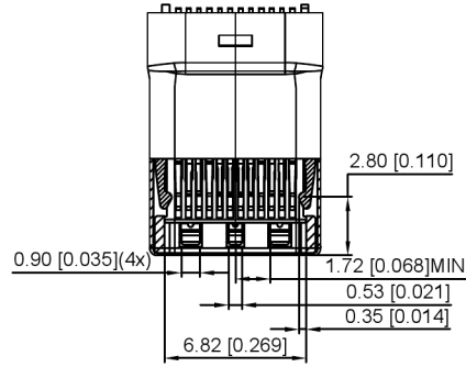
SECT B-B
