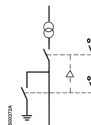
Mechanical interlock
