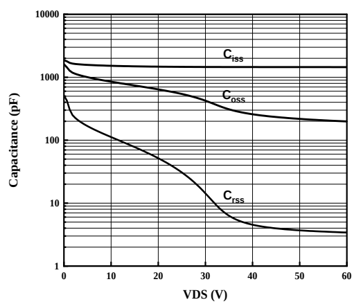
Fig5. Typical Capacitance
