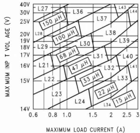
LM2596HV-12
