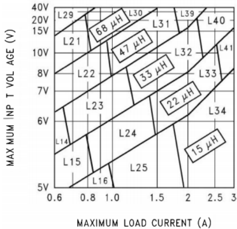
LM2596HV-3.3
