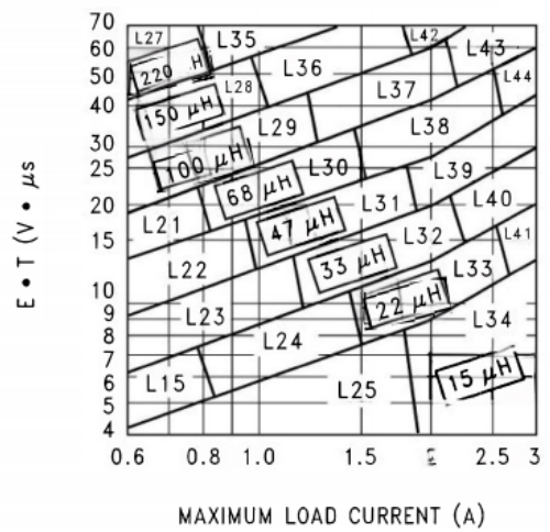
LM2596HV-12
