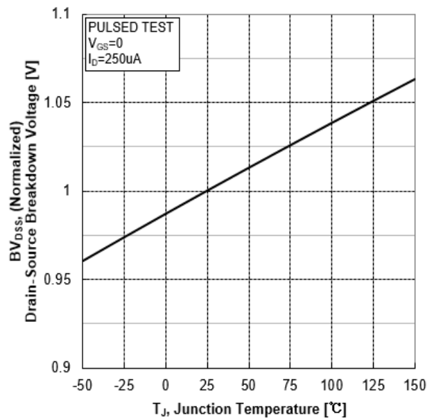
Figure 8. Normalized Breakdown Voltage vs Junction Temperature
