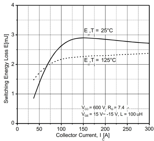
Typical Diode Switching Loss
