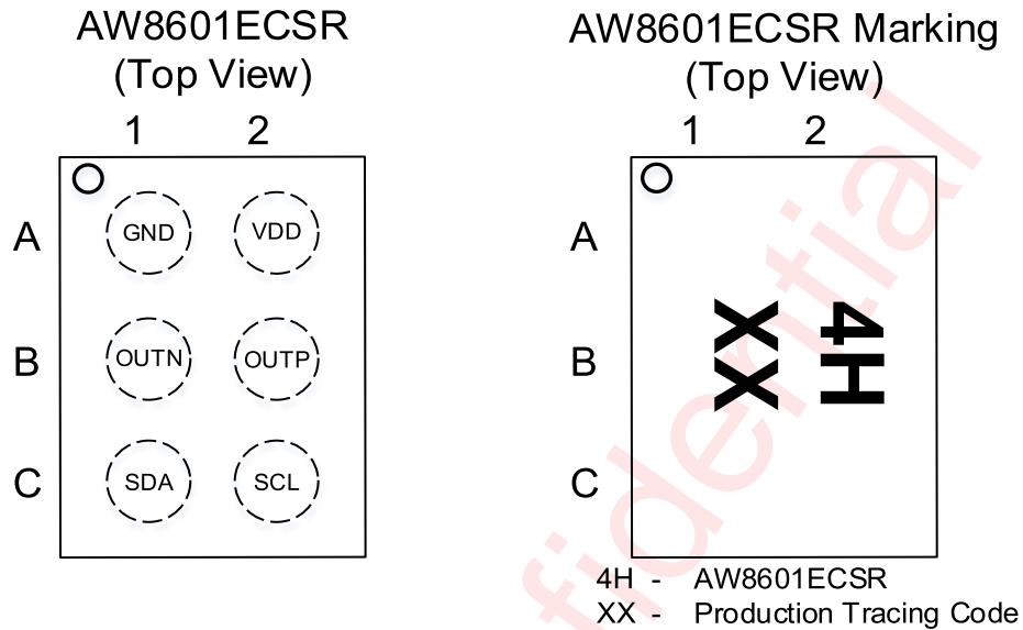
Figure 1 AW8601ECSR Pin Configuration and Top Mark
