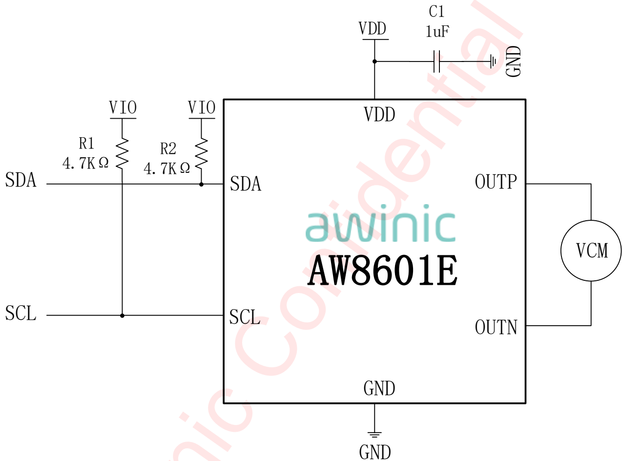
Figure 3 Typical Application Circuit of AW8601E
