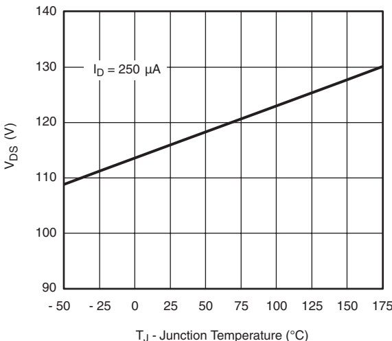
T_J - Drain-Source Breakdown vs. Junction-Temperature
