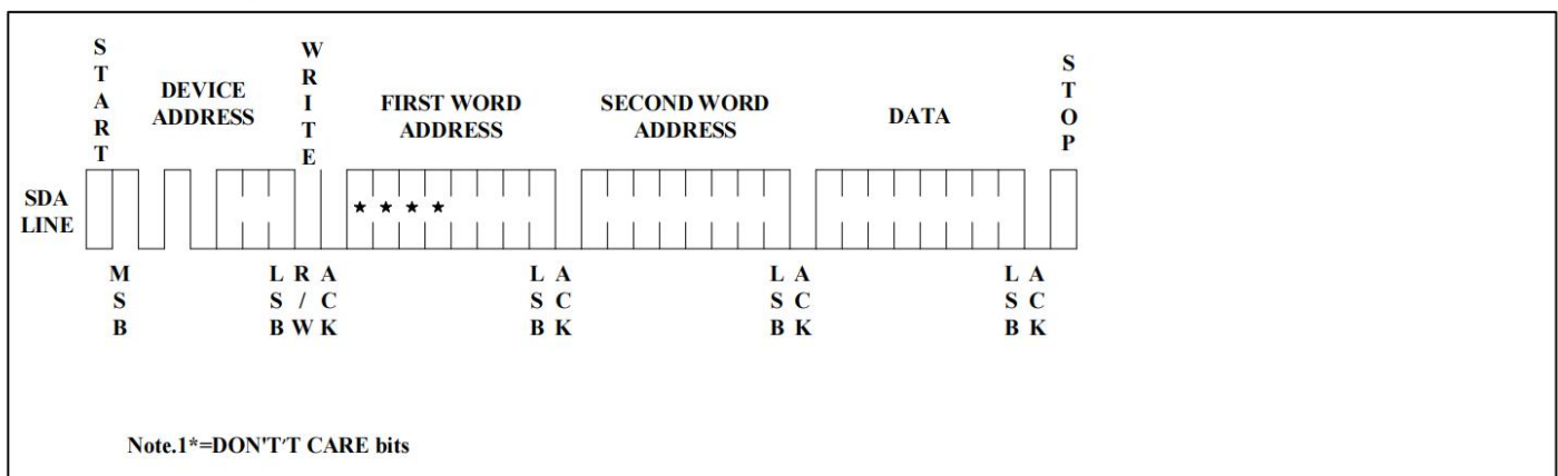
Figure 6. Byte Write
