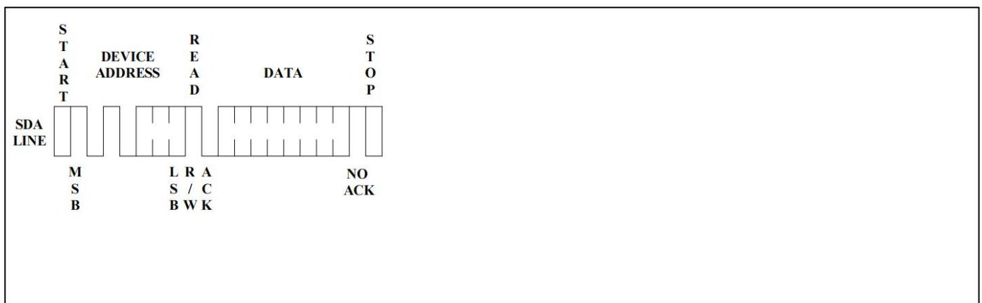
Figure 8. Current Address Read
