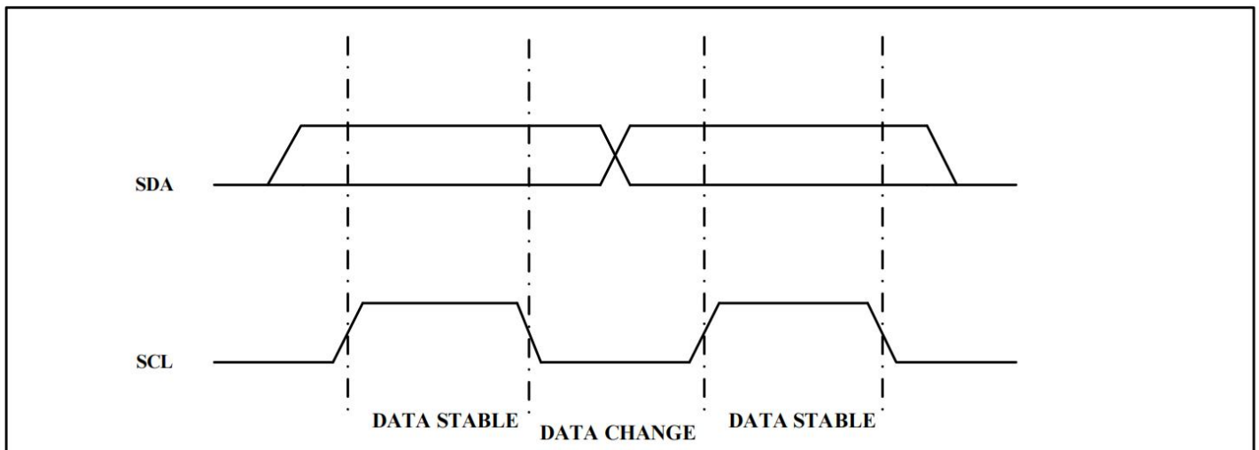
Figure 2. Data Validity
