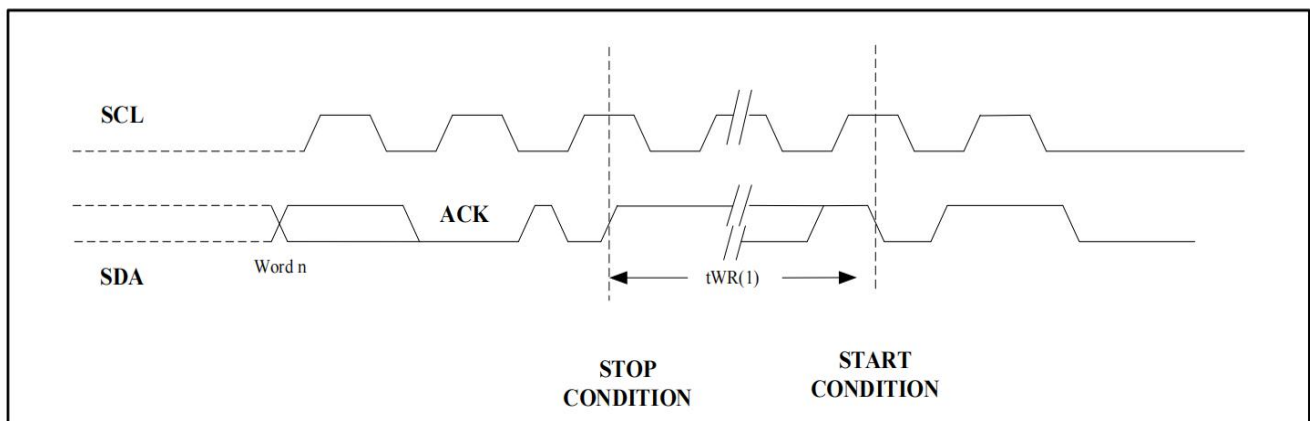
Figure 12. SCL: Serial Clock, SDA: Serial Data I/O
