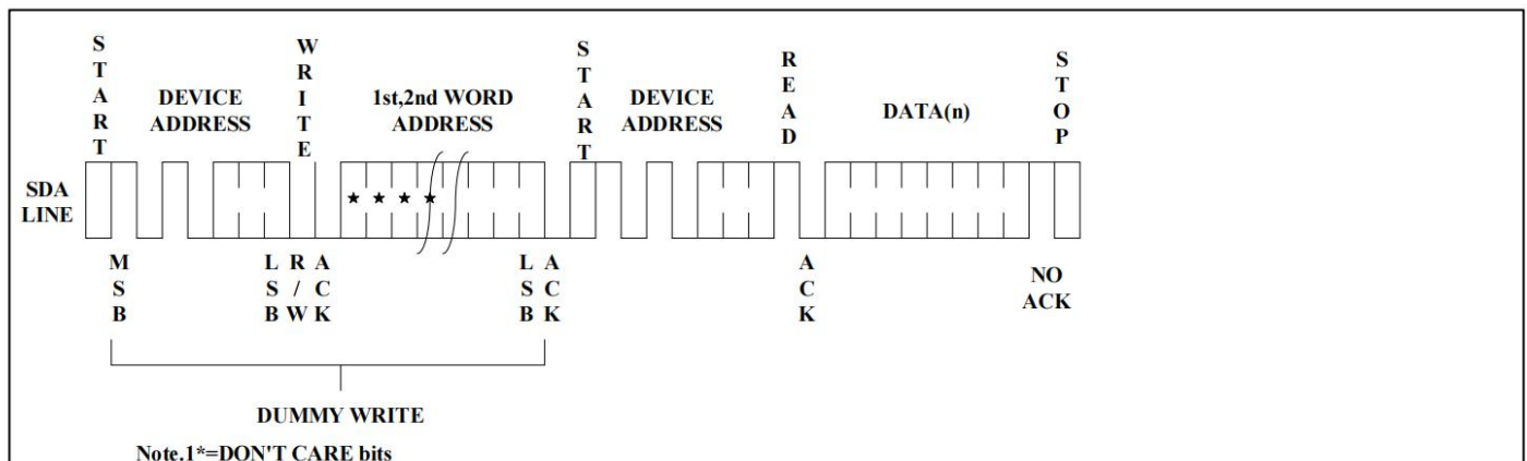
Figure 9. Random Read
