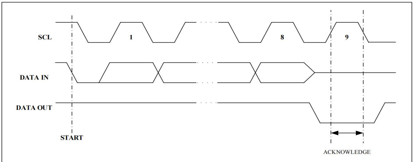
Figure 4. Output Acknowledge
