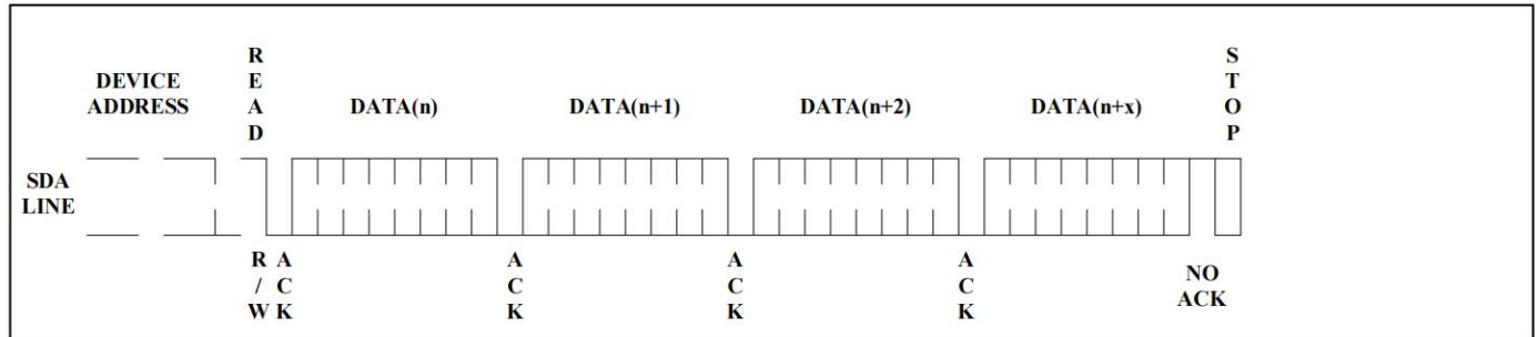
Figure 10. Sequential Read
