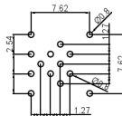
Pcb plate opening size (PCB板开孔尺寸)
