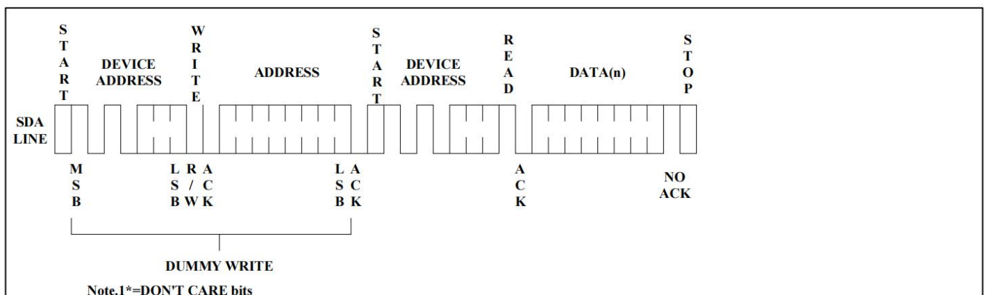
Figure 10. Random Read
