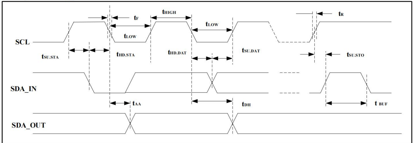
Figure 12. SCL: Serial Clock, SDA: Serial Data I/O
