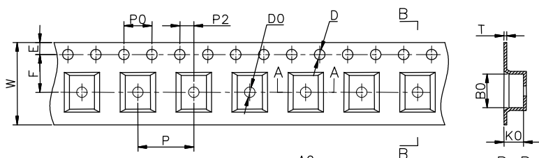
SMD-tape according to IEC 60286-3
