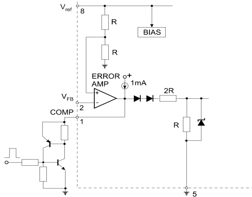
Figure 5. Latched Shutdown
