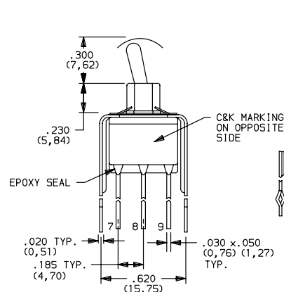
SNAP-IN
