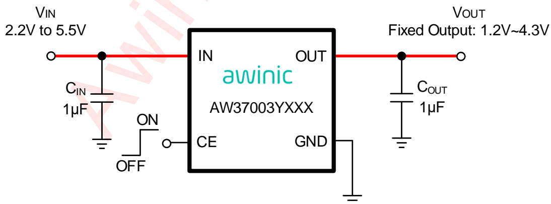
AW37003YXXX Application Circuit
