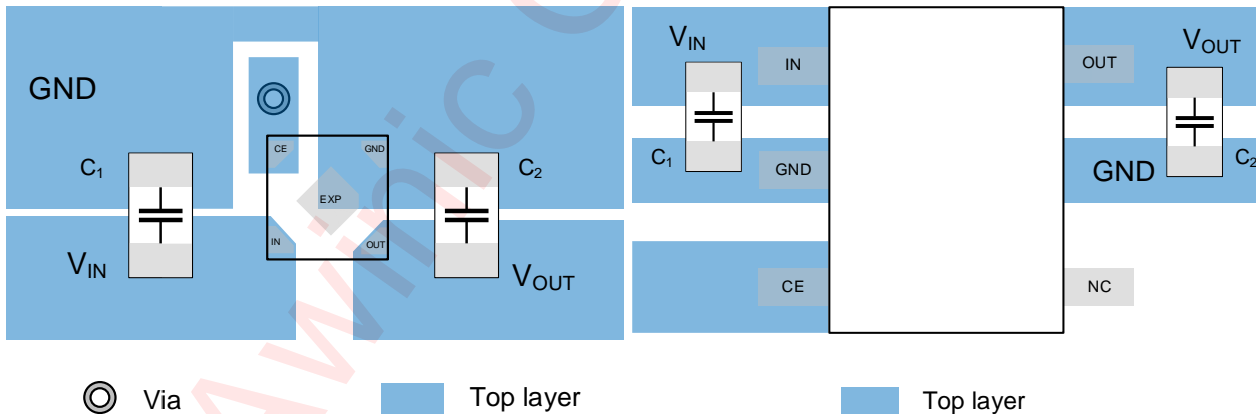
AW37003YXXX PCB LAYOUT
