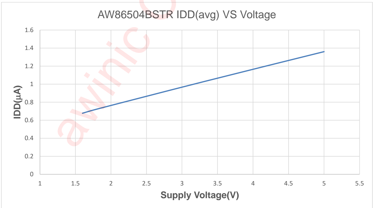
Average Supply Current vs. Supply Voltage(Ta=27°C)
