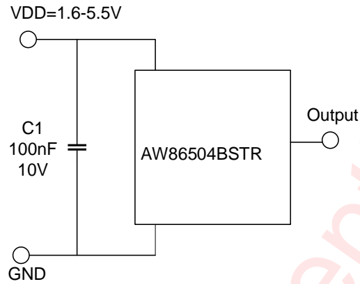
Figure 6 The Application Circuit of AW86504BSTR
