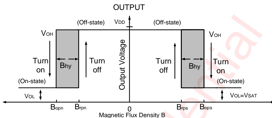
Figure 4 The Working Process of AW86504BSTR
