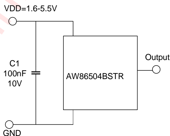
Figure 1 Typical Application Circuit of AW86504BSTR
