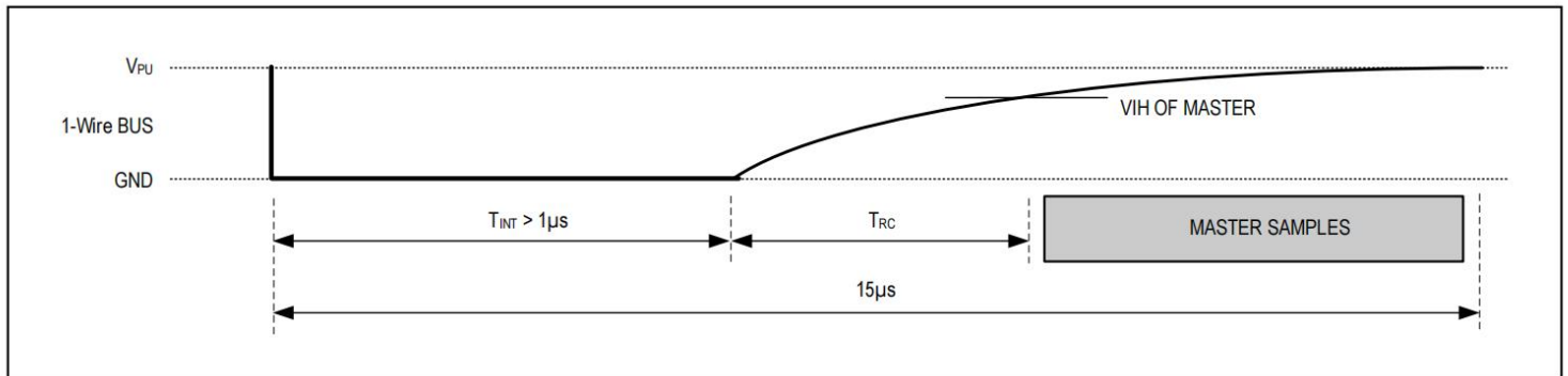
Figure 17. Detailed Master Read 1 Timing
