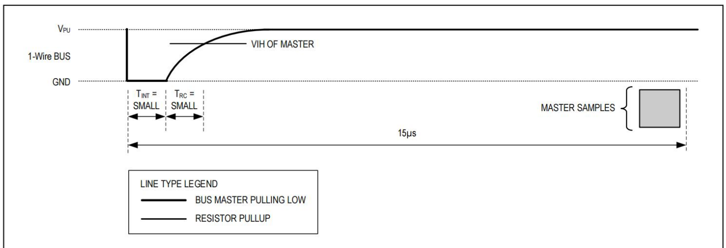
Figure 18. Recommended Master Read 1 Timing
