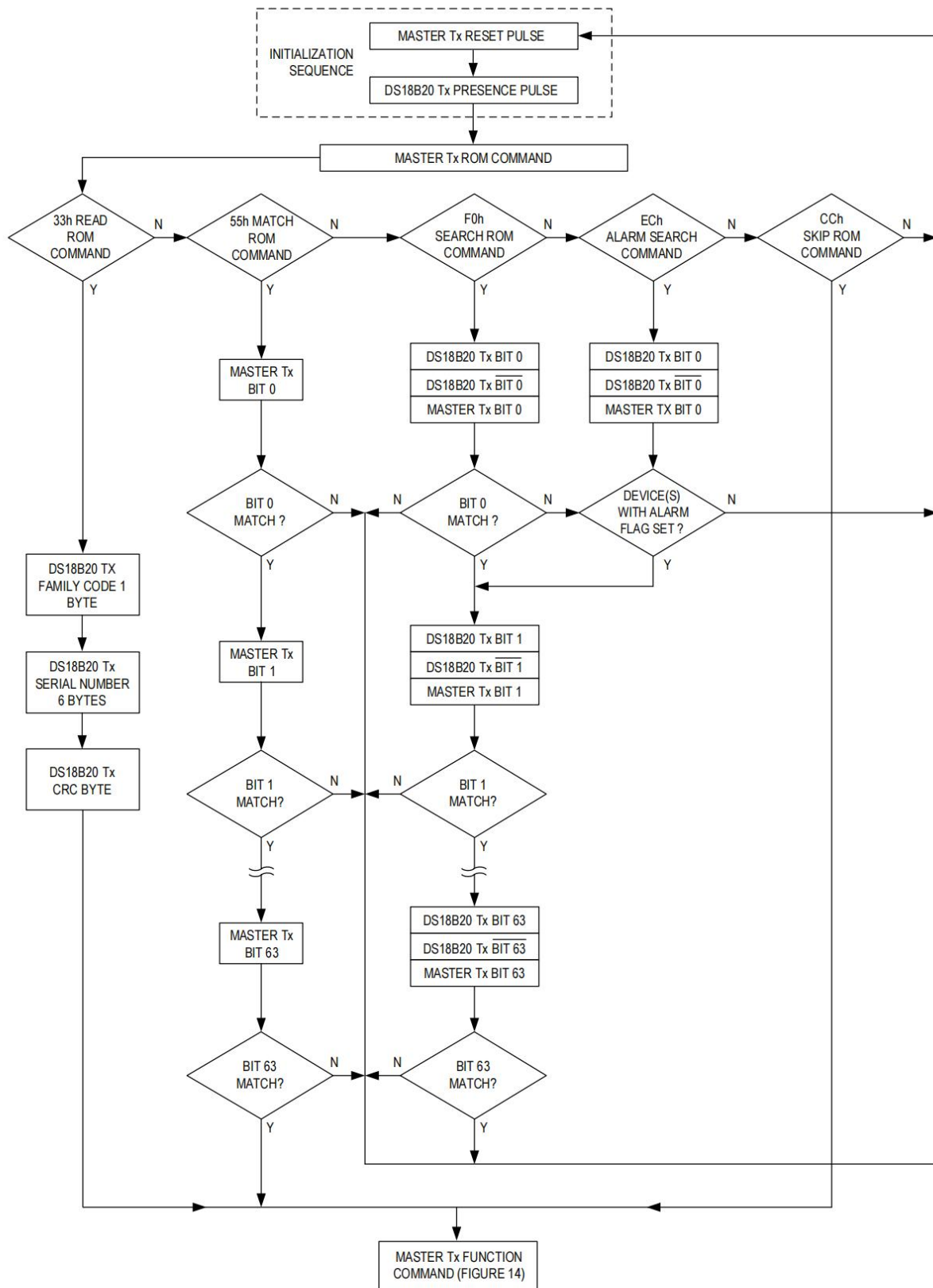
Figure 13. ROM Commands Flowchart
