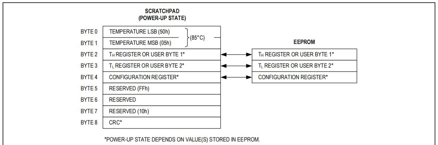
Figure 9. DS18B20 Memory Map
