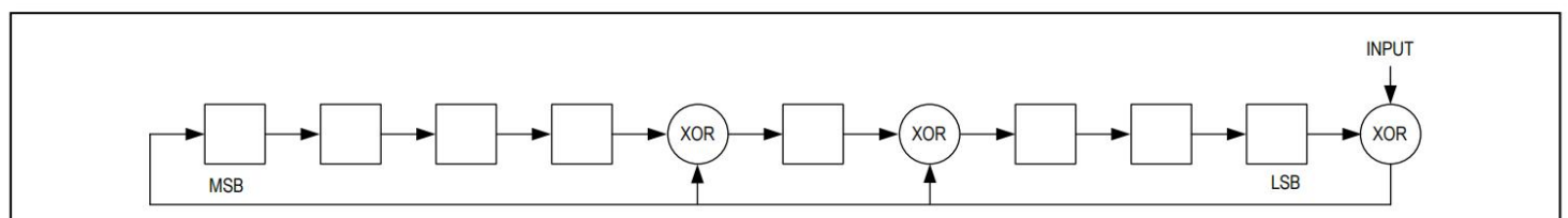
Figure 11. CRC Generator
