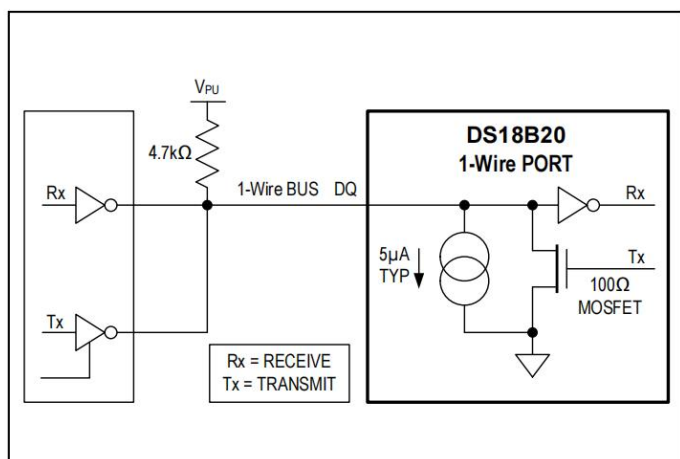
Figure 12. Hardware Configuration
