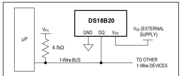
Figure 7. Powering the DS18B20 with an External Supply
