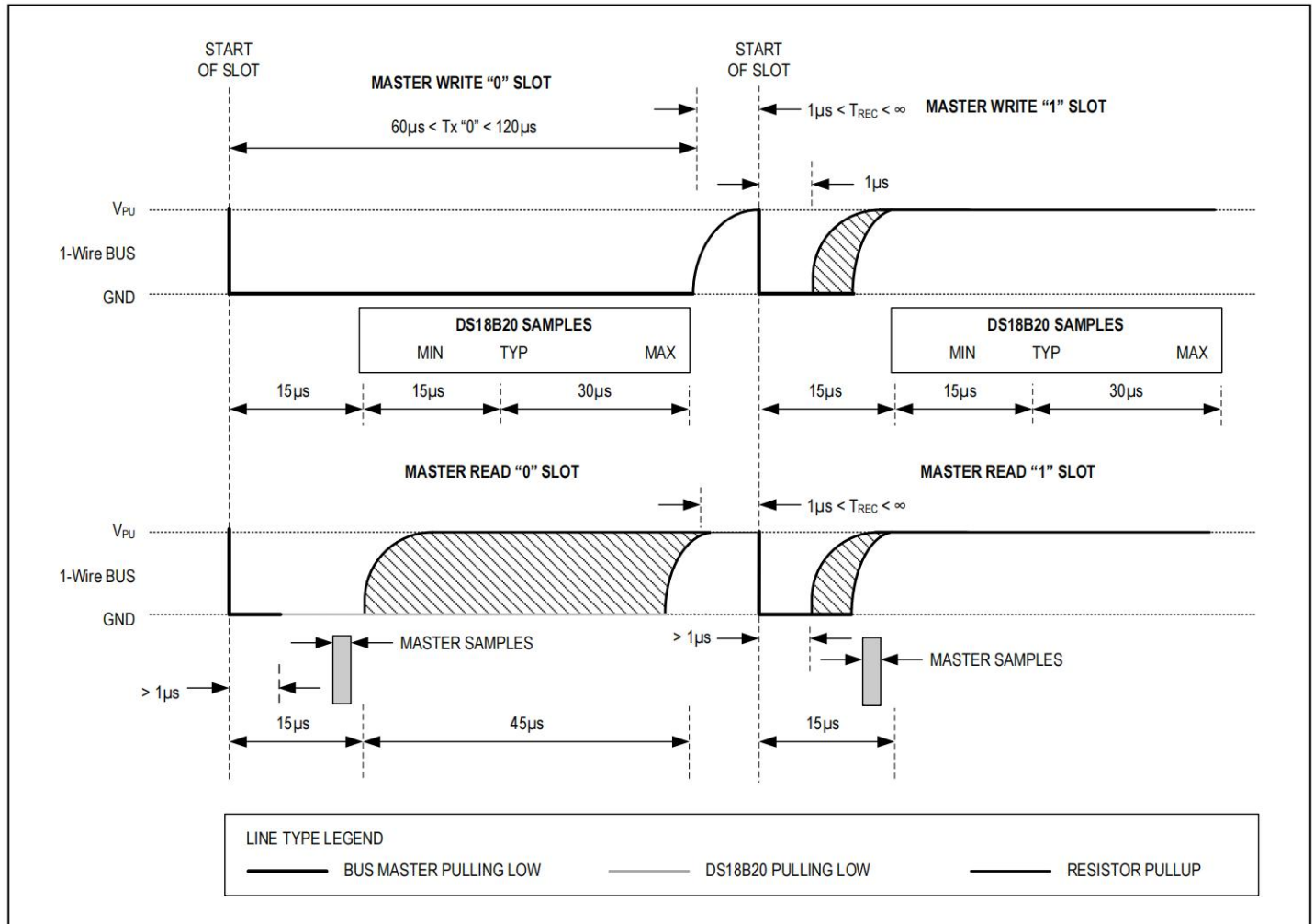
Figure 16. Read/Write Time Slot Timing Diagram
