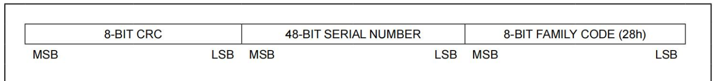
Figure 8. 64-Bit Lasered ROM Code
