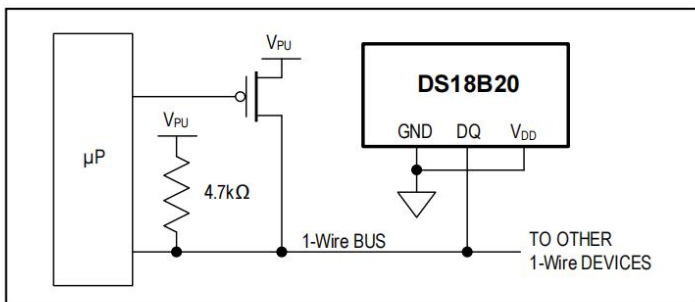
Figure 6. Supplying the Parasite-Powered DS18B20 During Temperature Conversions
