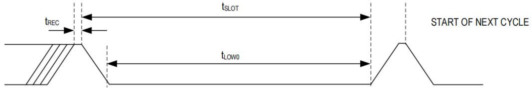
1-WIRE READ ZERO TIME SLOT
