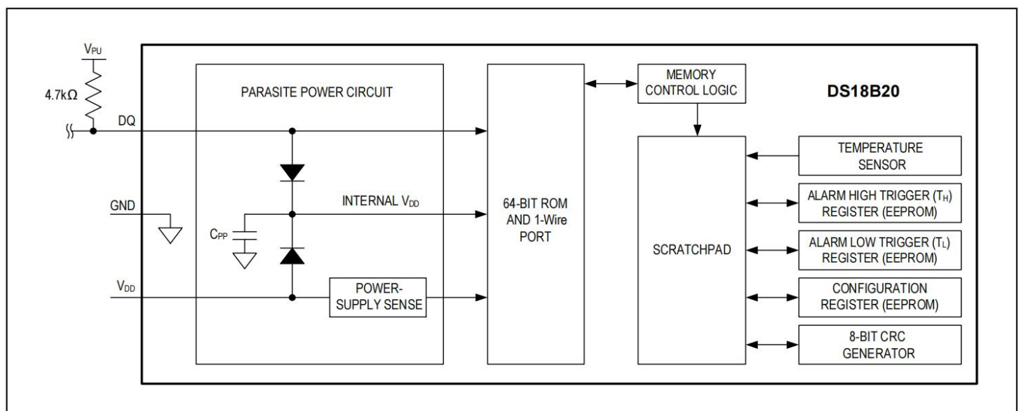
Figure 3. DS18B20 Block Diagram
