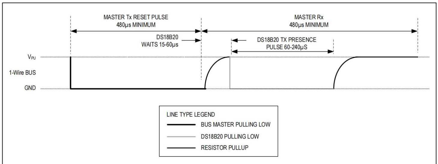
Figure 15. Initialization Timing
