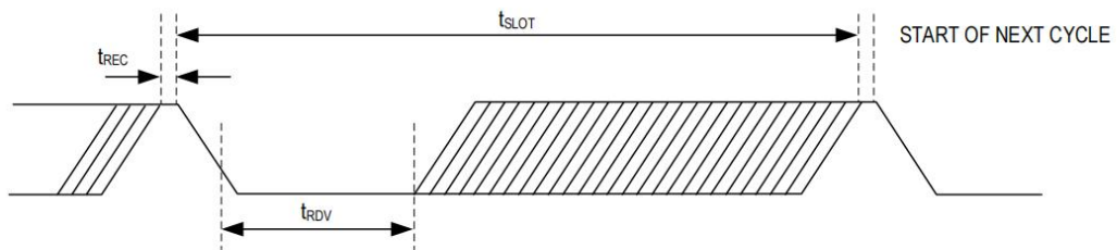
1-WIRE RESET PULSE
