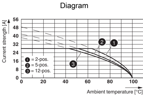
Type: PC 5/...-STF1-7,62 with PC 4/...-G-7,62 and BF-PC 4 Conductor cross section: 4 mm²
