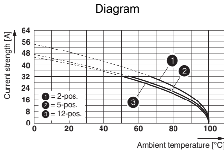
Type: PC 5/...-STF1-7,62 with PC 5/...-GF-7,62 Conductor cross section: 6 mm²
