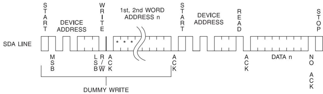
Figure 11. Random Read
