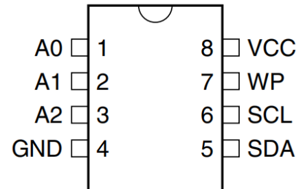
8-lead PDIP
