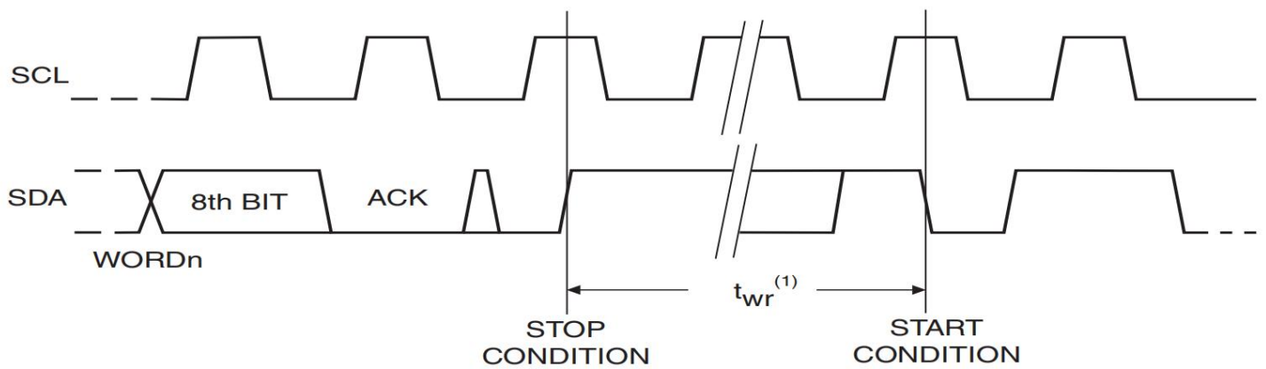
Figure 3. Write Cycle Timing
