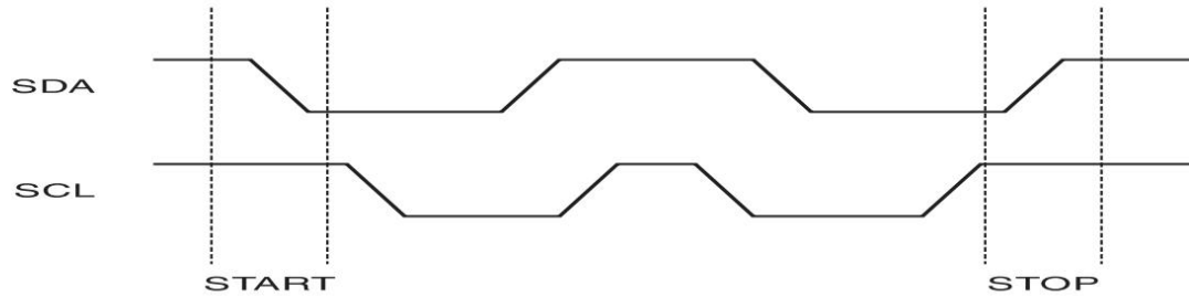
Figure 5. Start and Stop Definition
