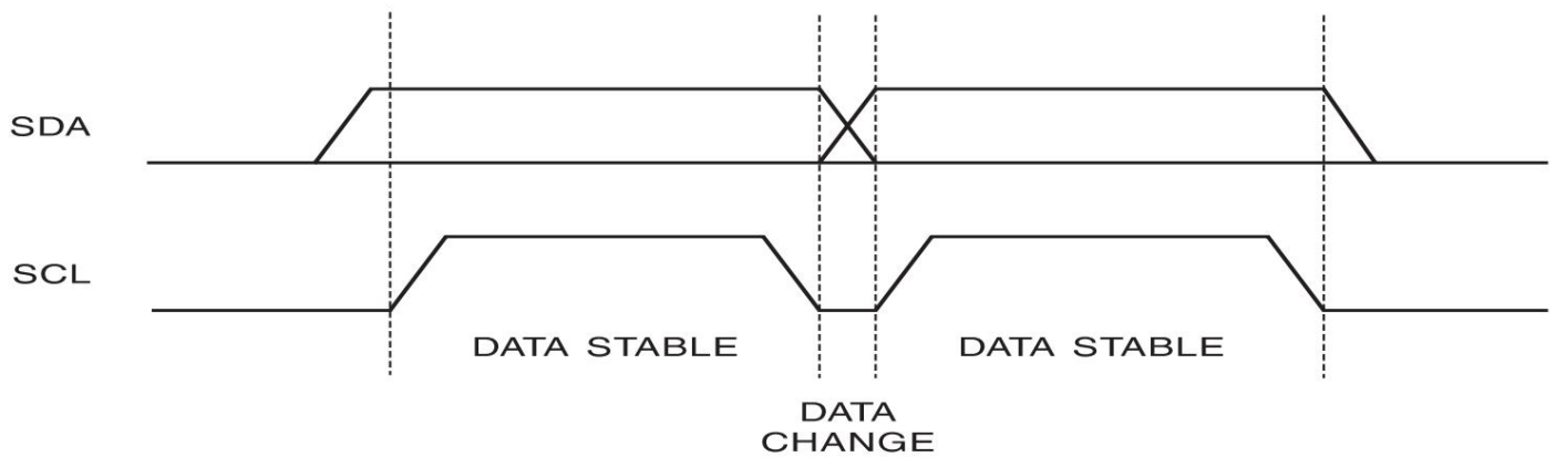
Figure 4. Data Validity
