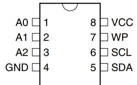
8-lead PDIP
