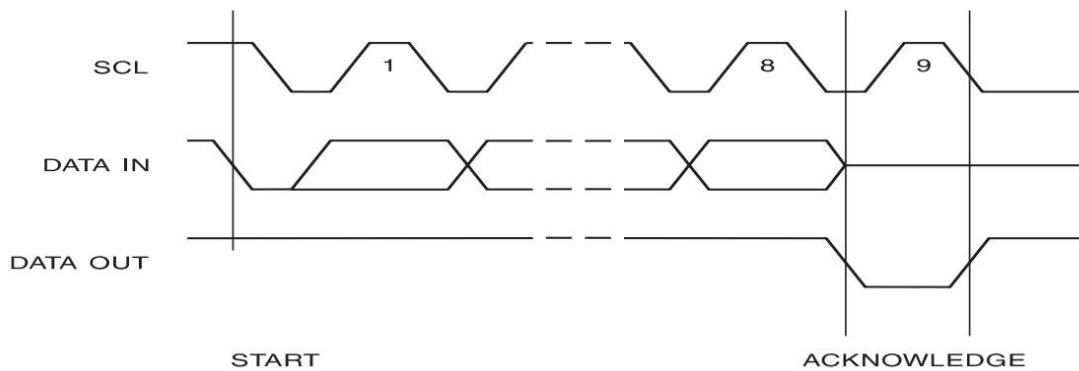
Figure 6. Output Acknowledge
