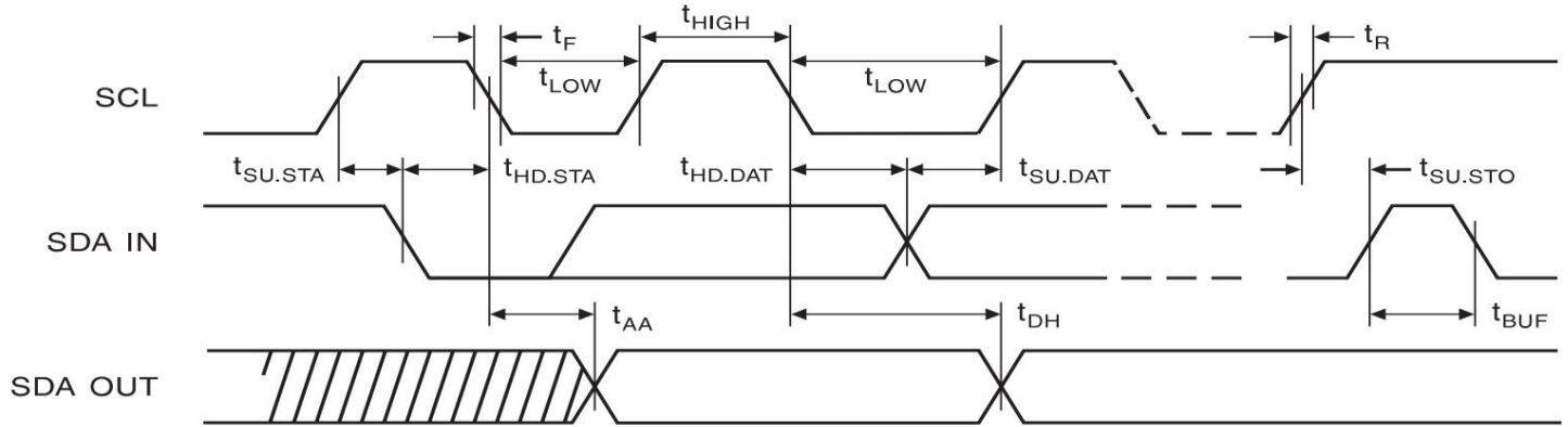
Figure 3. Write Cycle Timing
