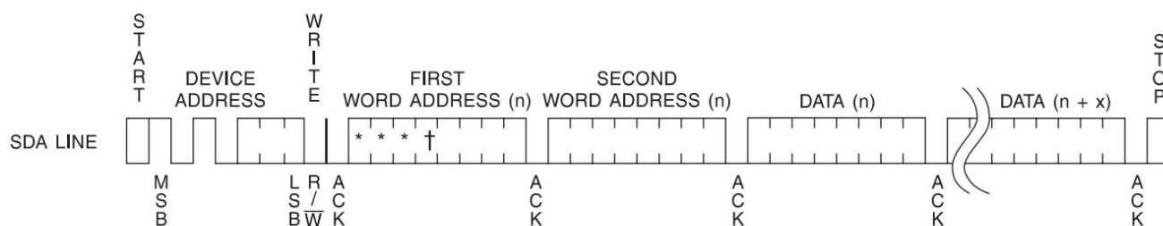
Figure 9. Page Write
