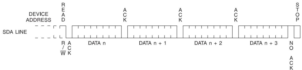
Figure 12. Sequential Read
