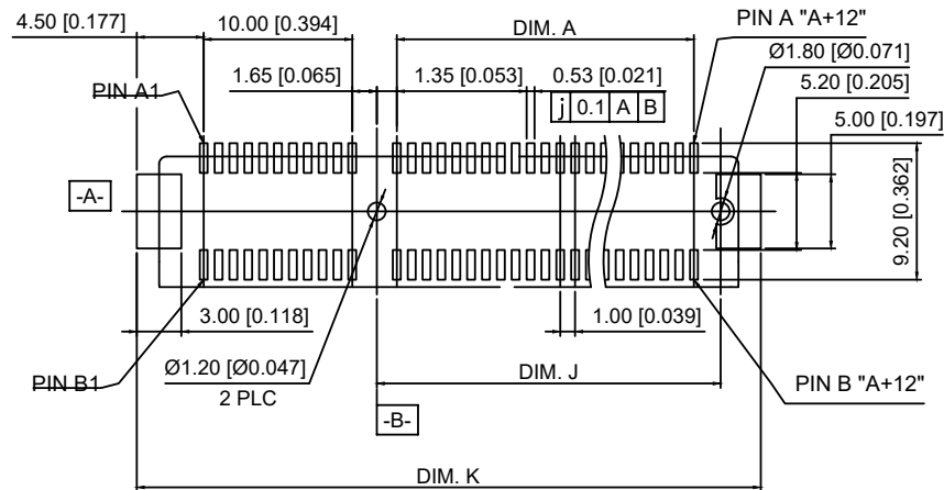
RECOMMENDED PCB LAYOUT (COMPONENT SIDE) TOLERANCE: ±0.05
