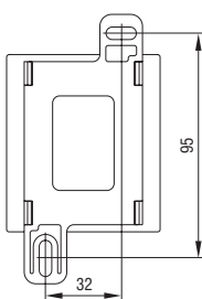
Screw fixing
