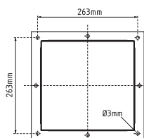
Drilling template for mounting frame
