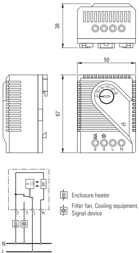
Heater
