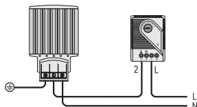
Heater
