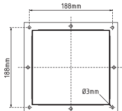
Drilling template for mounting frame
