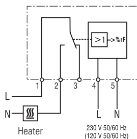
Connection diagram
