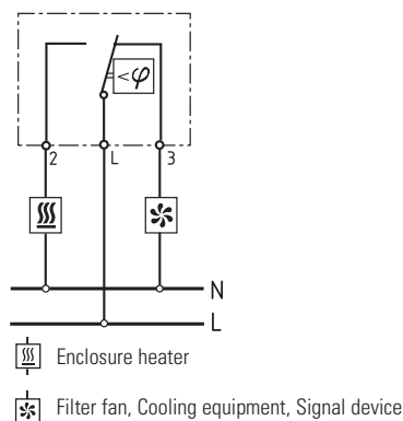
Connection diagram
