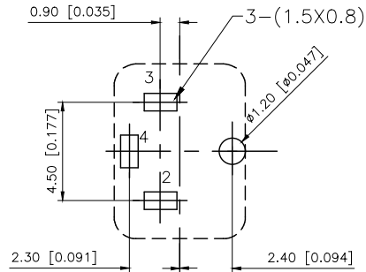
P.C.B LAYOUT MOUNTING PATTERN (TOP VIEW)
