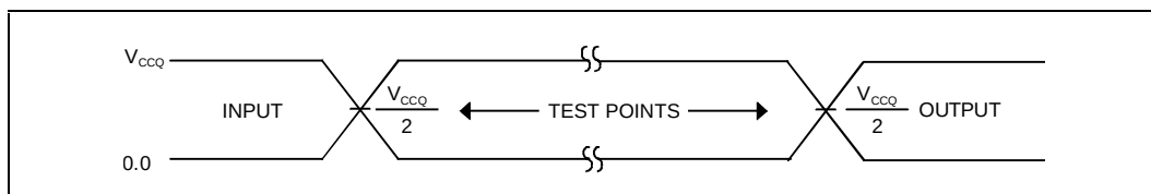
Figure 6. Input/Output Reference Waveform
