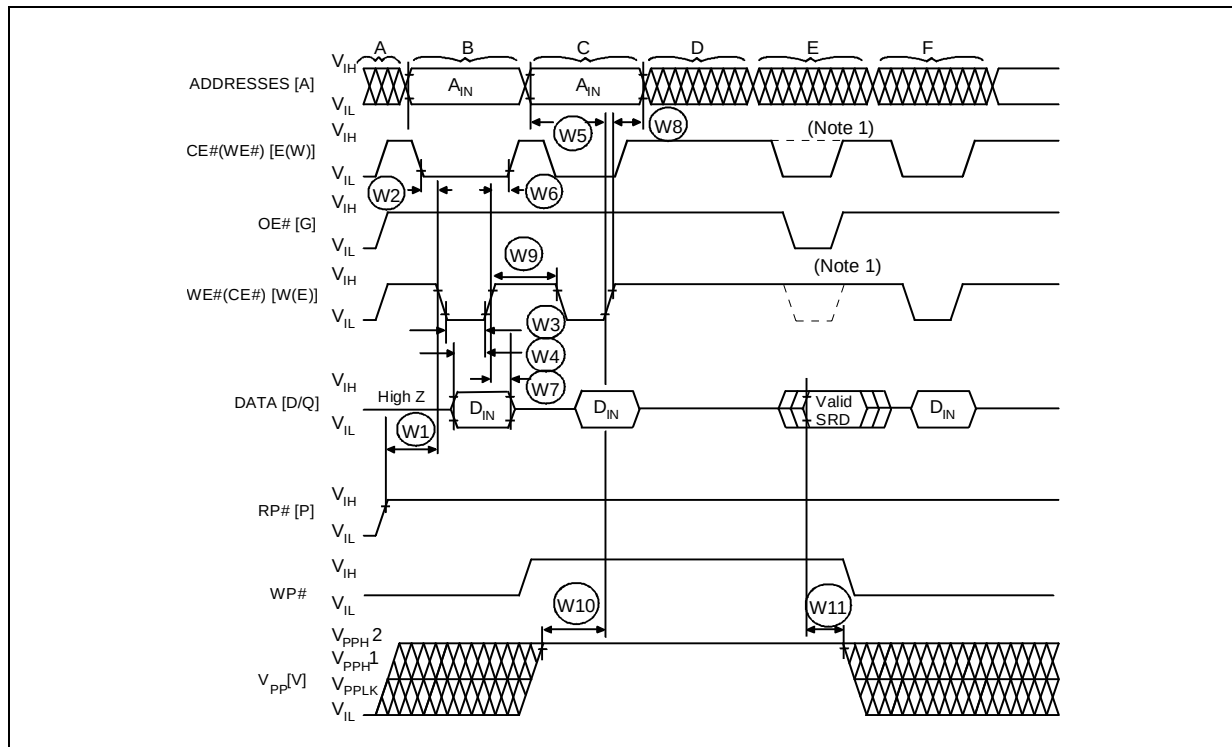
Figure 9. AC Waveform: Program and Erase Operations
