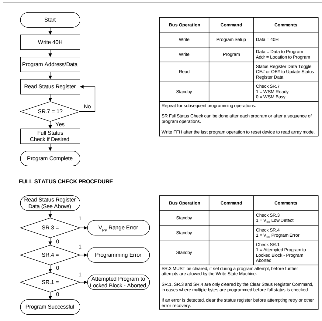
Figure 11. Program Flowchart
