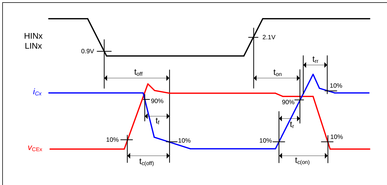
Figure 11 Switching times definition
