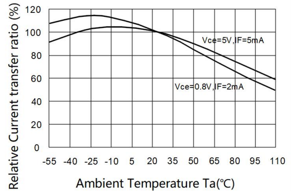
Fig.4 Relative Current Transte vs. Ambient Temperature
