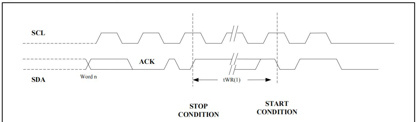
Figure 11: SCL: Serial Clock, SDA: Serial Data I/O
