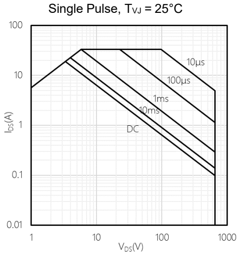
Figure 1. Safe operating area (SOA)
