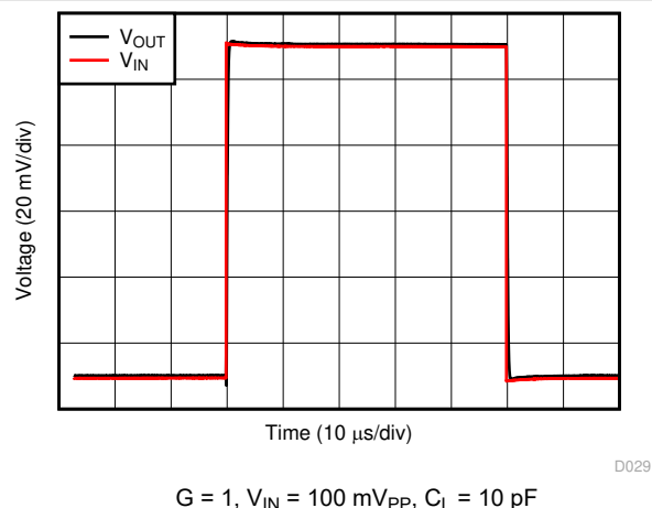
Figure 6-24. Small-Signal Step Response
