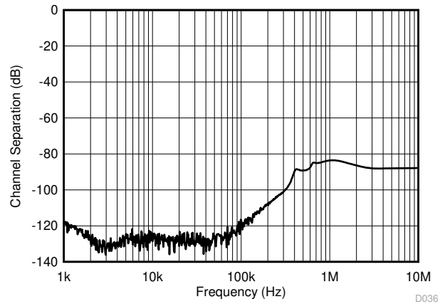
Figure 6-31. Channel Separation
