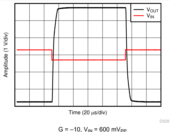
Figure 6-23. Overload Recovery
