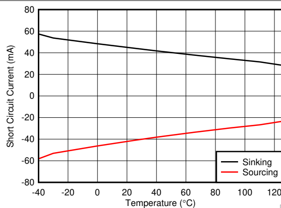
Figure 6-28. Short-Circuit Current vs Temperature
