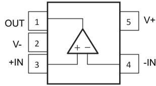
Figure 5-1. 5-Pin SOT-23 DBV Package (LMV321A Top View)
