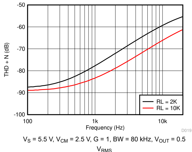
Figure 6-14. THD + N vs Frequency
