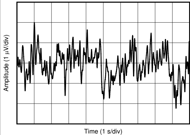
Figure 6-12. 0.1 Hz to 10 Hz Integrated Voltage Noise
