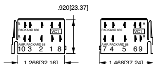
VC1 CONNECTOR HOUSING
