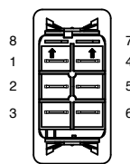
BOTTOM VIEW TERMINAL ARRANGEMENT 8 TERMINAL BASE
