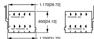
VCH CONNECTOR HOUSING
