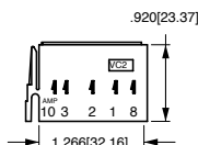
VC2 CONNECTOR HOUSING (For AMP terminals only)
