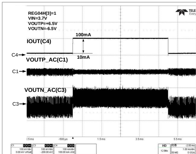
Figure 71 Load Transient(80mA Mode)
