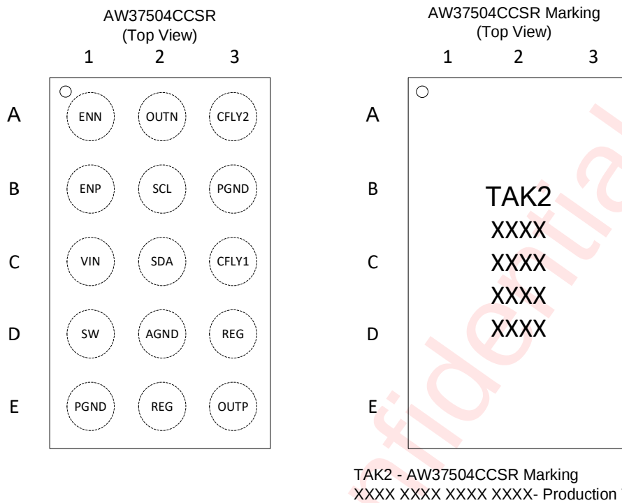
Figure 2 Pin Configuration and Top Mark
