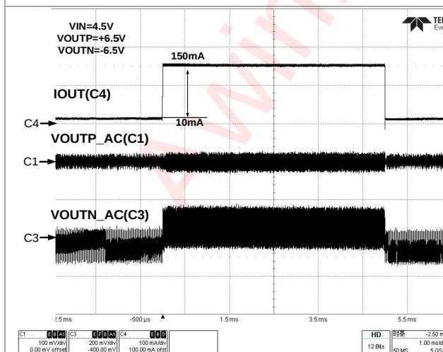
Figure 75 Load Transient(150mA Mode)
