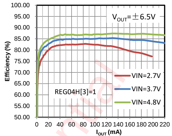
Figure 18 Efficiency (150mA Mode)
