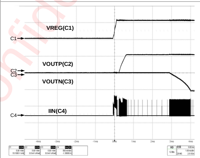
Figure 92 Inrush Current (Sequential)
