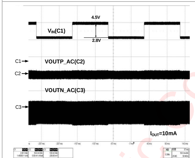
Figure 85 Line Transient (150mA Mode)
