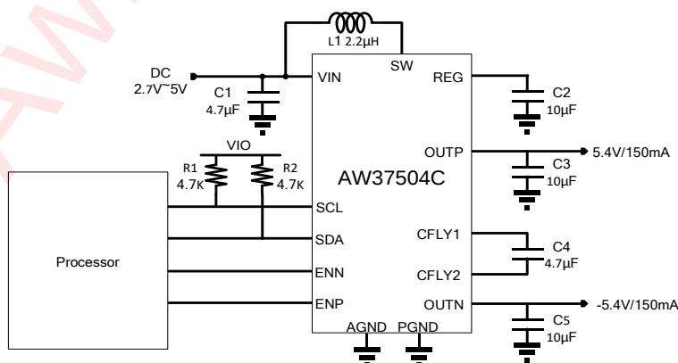
Figure 1 Typical Application Circuit of AW37504C
