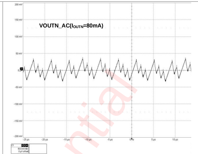
Figure 54 V OUTN Output Voltage Ripple(80mA Mode)
