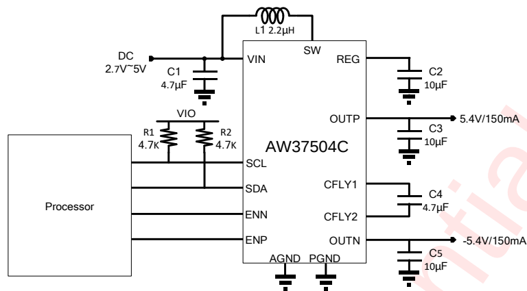
Figure 4 AW37504C Application circuit
