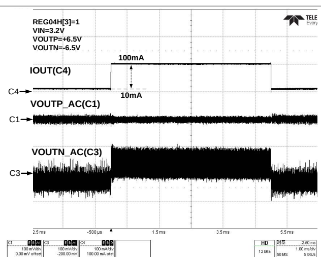
Figure 70 Load Transient(80mA Mode)
