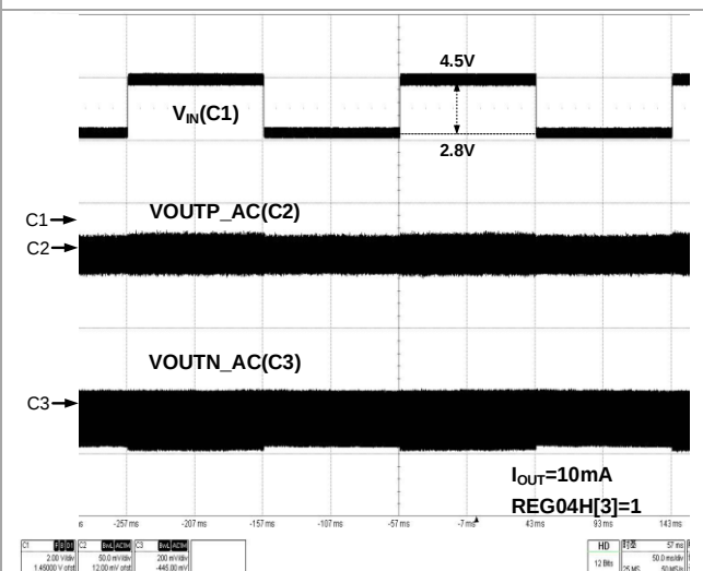
Figure 88 Line Transient (150mA Mode)
