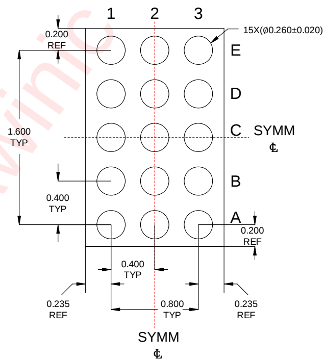
Bottom View
