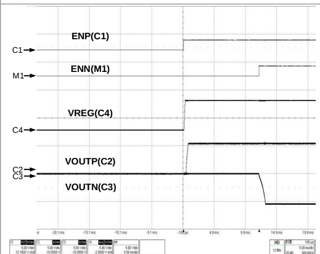
Figure 94 Power Up Sequencing (Sequential)
