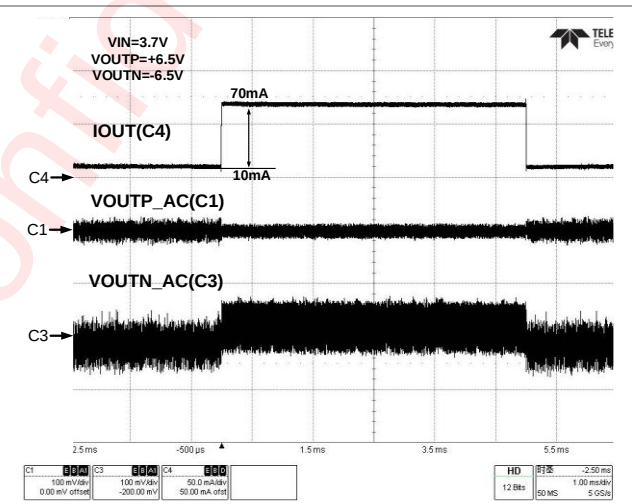
Figure 68 Load Transient(80mA Mode)
