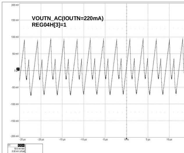
Figure 65 V OUTN Output Voltage Ripple(150mA Mode)
