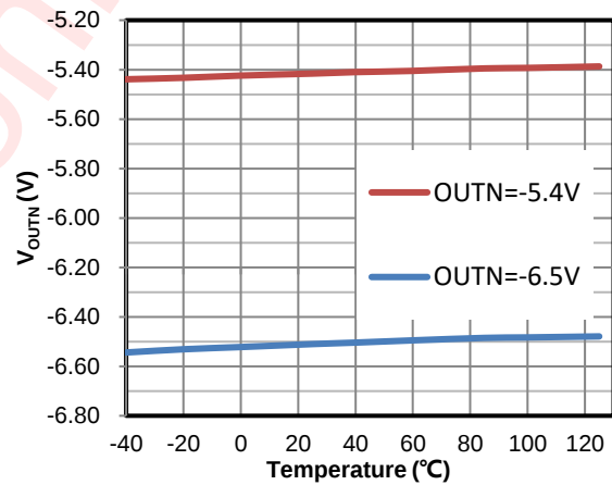
Figure 9 V_{OUTN} vs. Temperature
