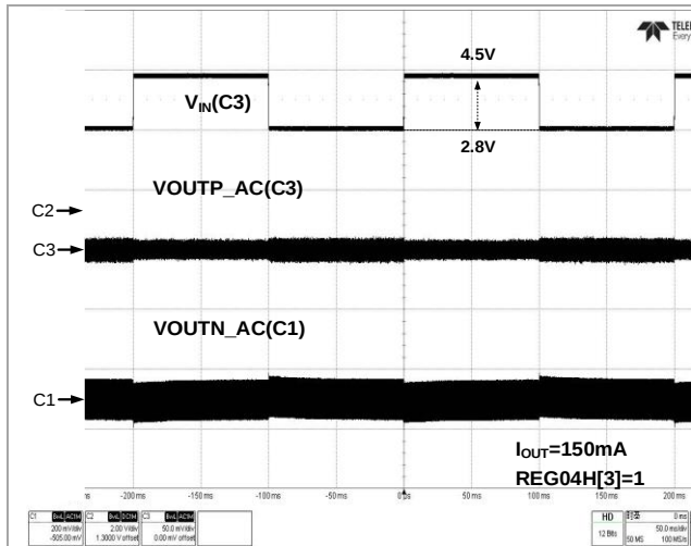
Figure 89 Line Transient (150mA Mode)
