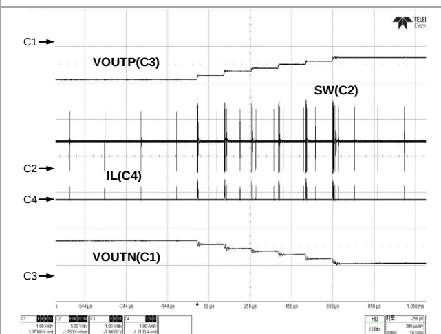
Figure 100 Ramp Up (V OUTP And V OUTN )
