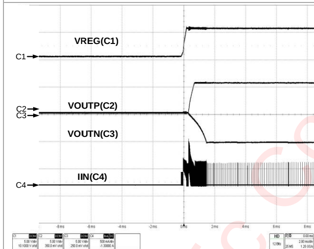
Figure 91 Inrush Current (Simultaneous)
