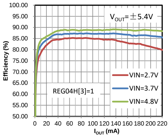
Figure 17 Efficiency (150mA Mode)
