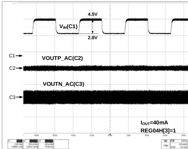
Figure 83 Line Transient (80mA Mode)
