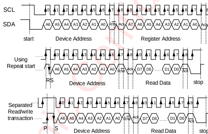
Figure 108 I²C Read Byte Cycle
