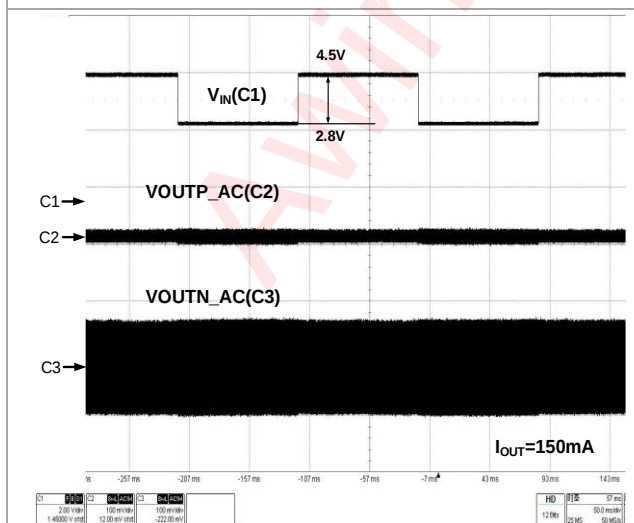
Figure 87 Line Transient (150mA Mode)
