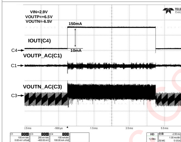
Figure 73 Load Transient(150mA Mode)
