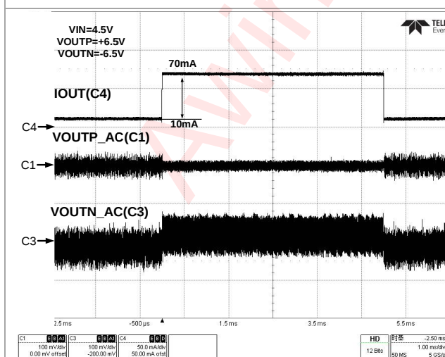
Figure 67 Load Transient(80mA Mode)
