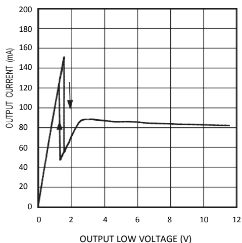
OUTPUT CURRENT vs. TRANSMITTER OUTPUT-LOW VOLTAGE
