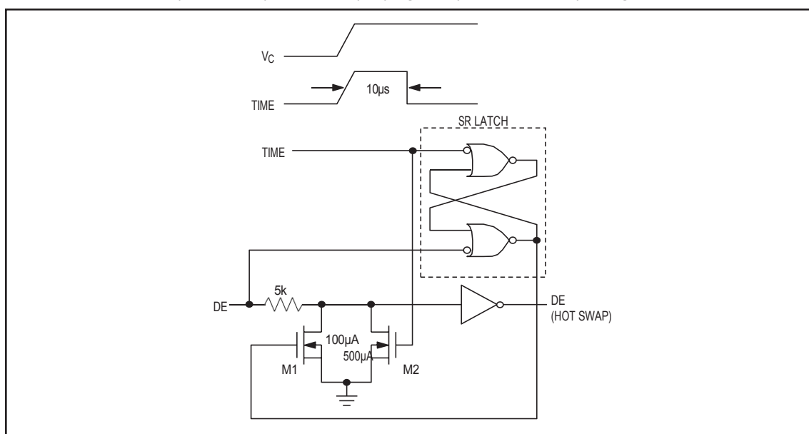
Figure 9. Simplified Structure of the Driver Enable Pin (DE)
