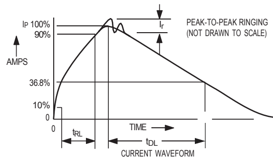
Figure 10b. Human Body Current Waveform
