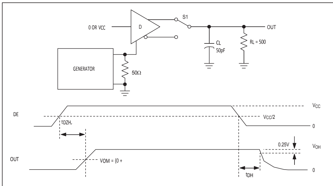
Figure 4. Driver Enable and Disable Times ( t_{DZH} , t_{DZH} , t_{DZH(SHDN)} )
