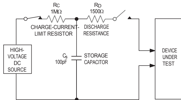
Figure 10a. Human Body ESD Test Model
