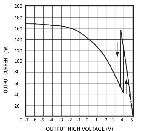
OUTPUT CURRENT vs. TRANSMITTER OUTPUT-HIGH VOLTAGE
