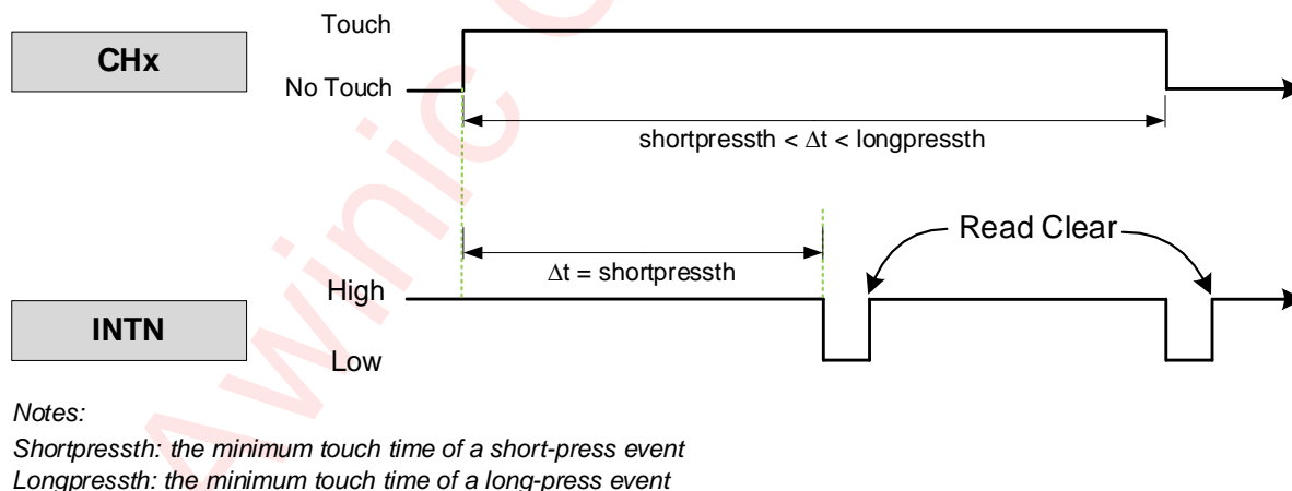
Figure 21 Short-press Sequence Diagram
