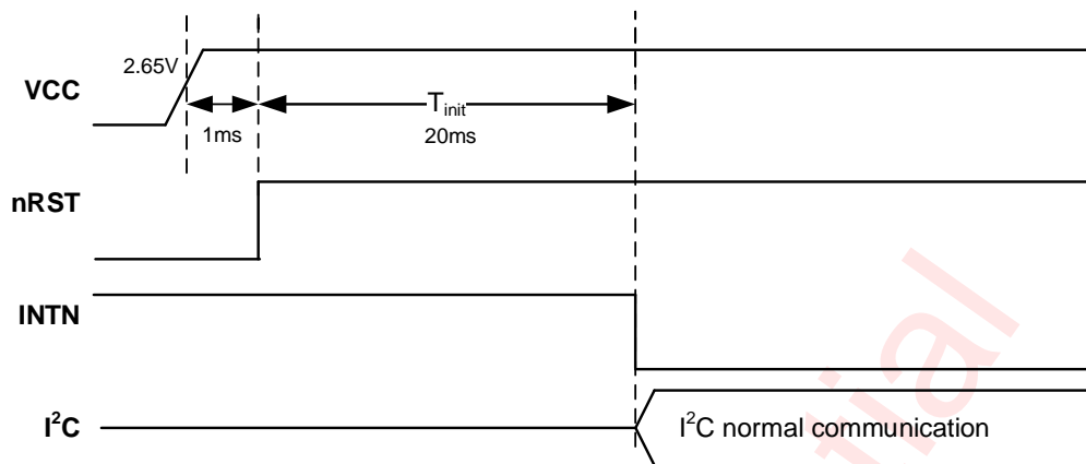
Figure 10 Power On Timing
