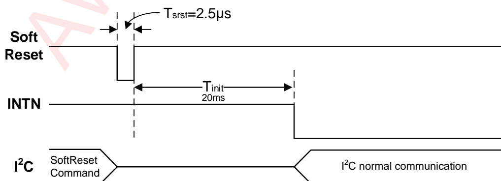
Figure 12 Soft Reset Timing
