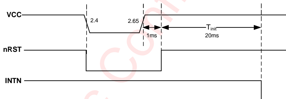
Figure 11 Brown Out Timing
