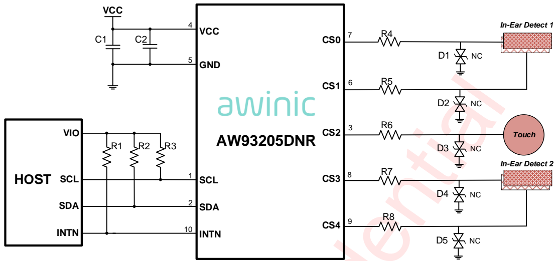
Figure 1 AW93205DNR Typical Application Circuit (touch and in-ear)
