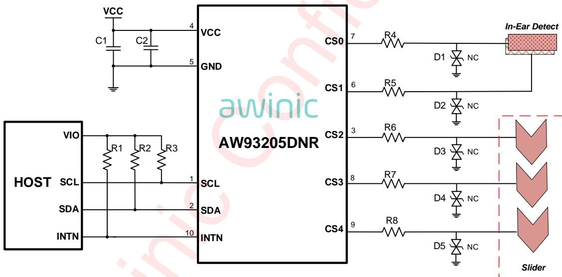
Figure 2 AW93205DNR Typical Application Circuit (in-ear and slide)
