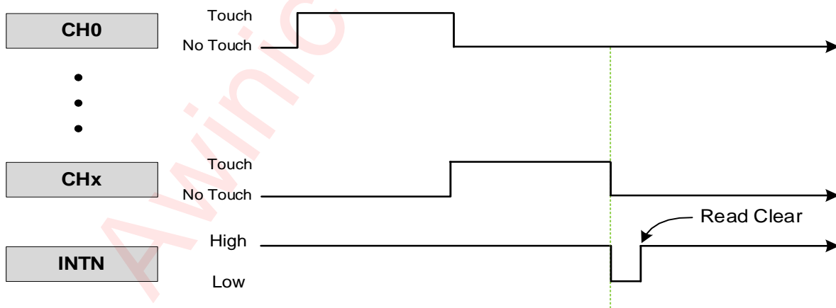
Figure 23 Slide Sequence Diagram
