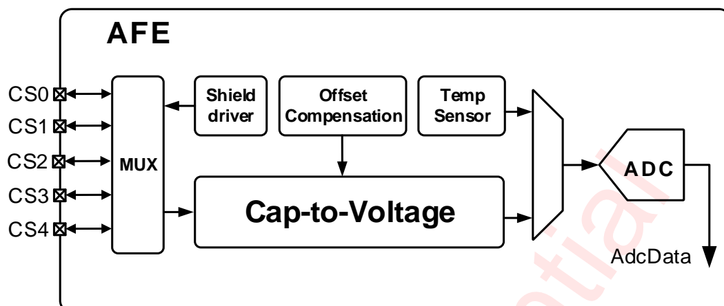
Figure 7 AFE Block Diagram
