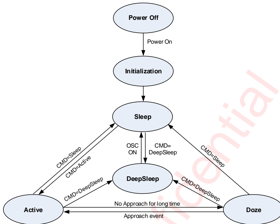
Figure 13 Operation Mode Switching
