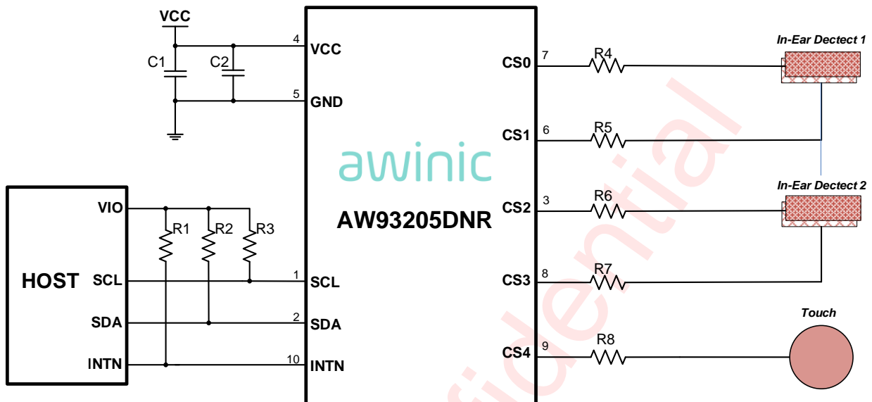
Figure 25 AW93205DNR Typical Application Circuit (two in-ears and a touch key)
