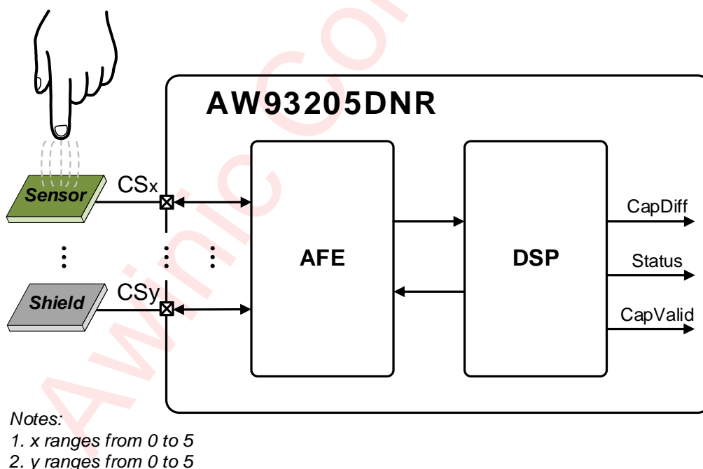
Figure 6 Proximity Sensor Operation Overview
