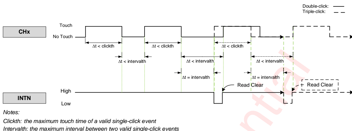
Figure 20 Double-click and Triple-click Sequence Diagram
