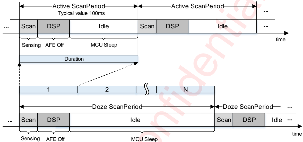
Figure 9 Active Mode and Doze Mode Scan Period
