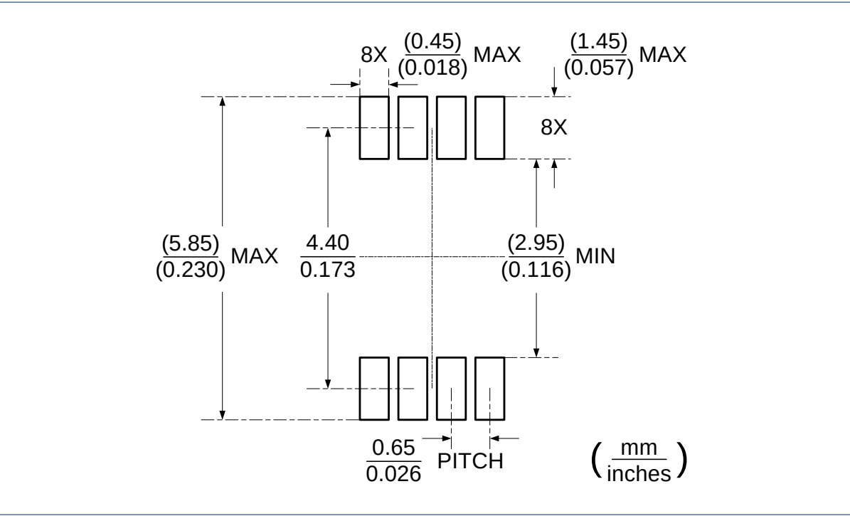
RECOMMENDED SOLDERING FOOTPRINT, MSOP-8L
