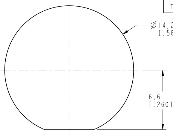
RECOMMENDED MOUNTING HOLE DIMENSIONS
