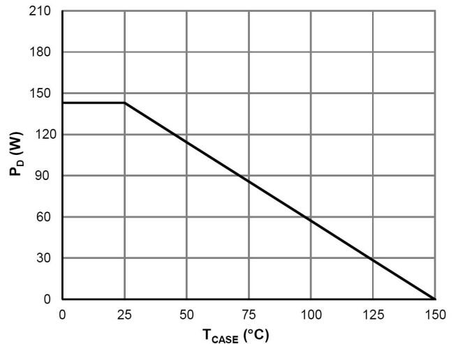
Power De-rating
